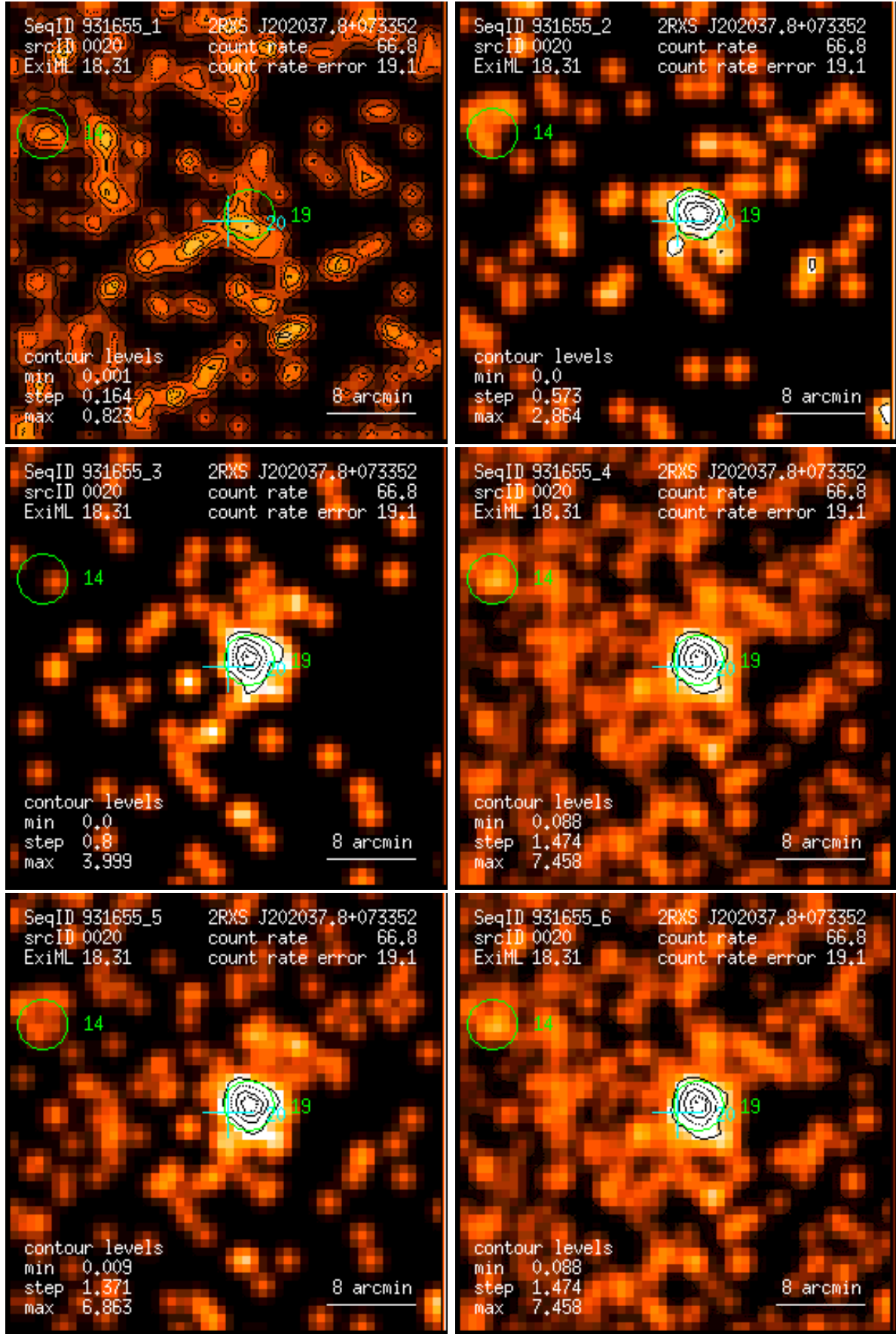
Figure 20: RASS 931655: detection 0020: band rate images, Gaussian filter: (1) PSPC channels 11 – 41, (2) 52 – 90, (3) 91 – 201, (4) 11 – 235, (5) 52 – 201, (6) 11 – 201. Broad band rates in counts/ks. Band rate contour levels in counts/ks/arcmin 2 .
