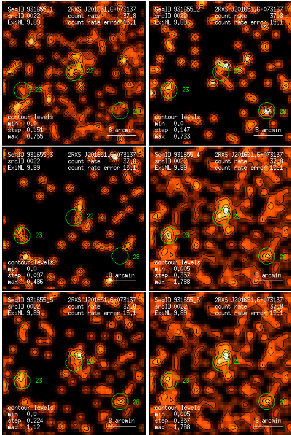
Figure 22: RASS 931655: detection 0022: band rate images, Gaussian filter: (1) PSPC channels 11 – 41, (2) 52 – 90, (3) 91 – 201, (4) 11 – 235, (5) 52 – 201, (6) 11 – 201. Broad band rates in counts/ks. Band rate contour levels in counts/ks/arcmin 2 .
