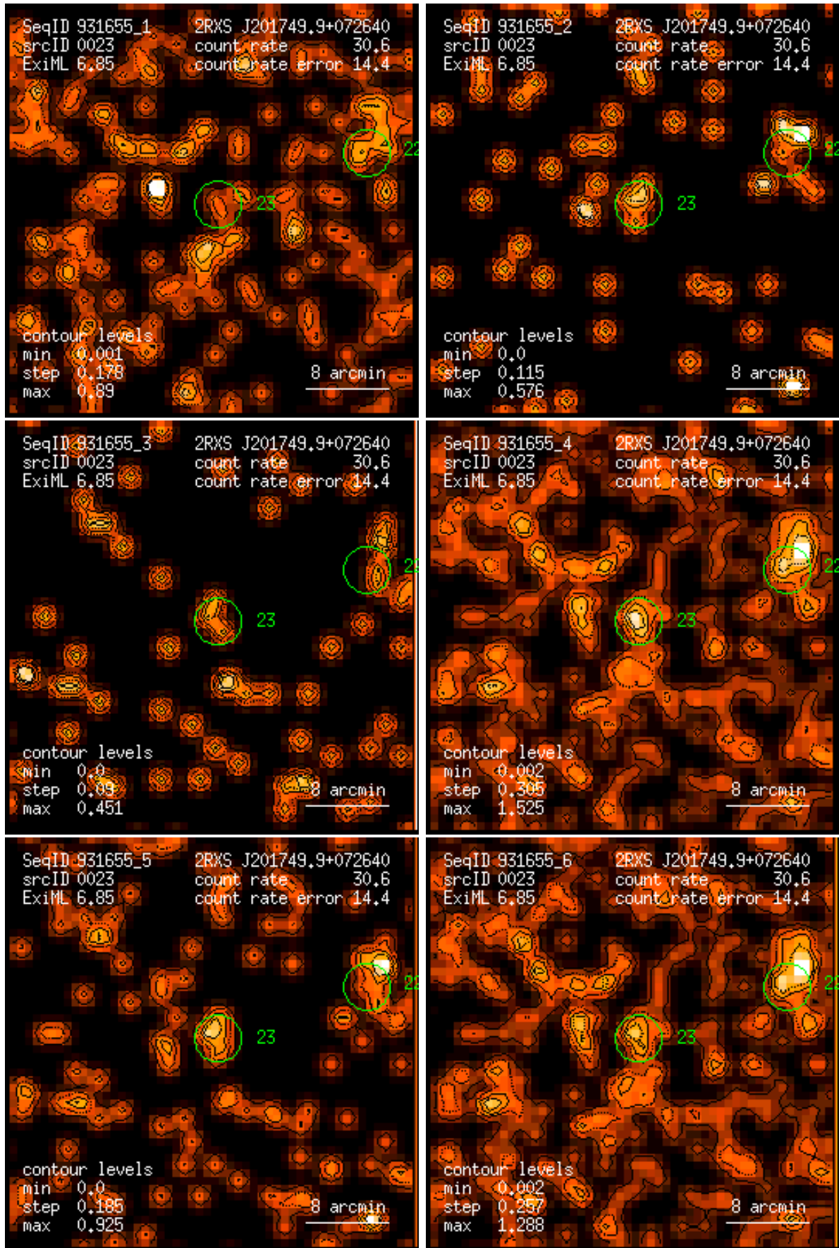
Figure 23: RASS 931655: detection 0023: band rate images, Gaussian filter: (1) PSPC channels 11 – 41, (2) 52 – 90, (3) 91 – 201, (4) 11 – 235, (5) 52 – 201, (6) 11 – 201. Broad band rates in counts/ks. Band rate contour levels in counts/ks/arcmin 2 .
