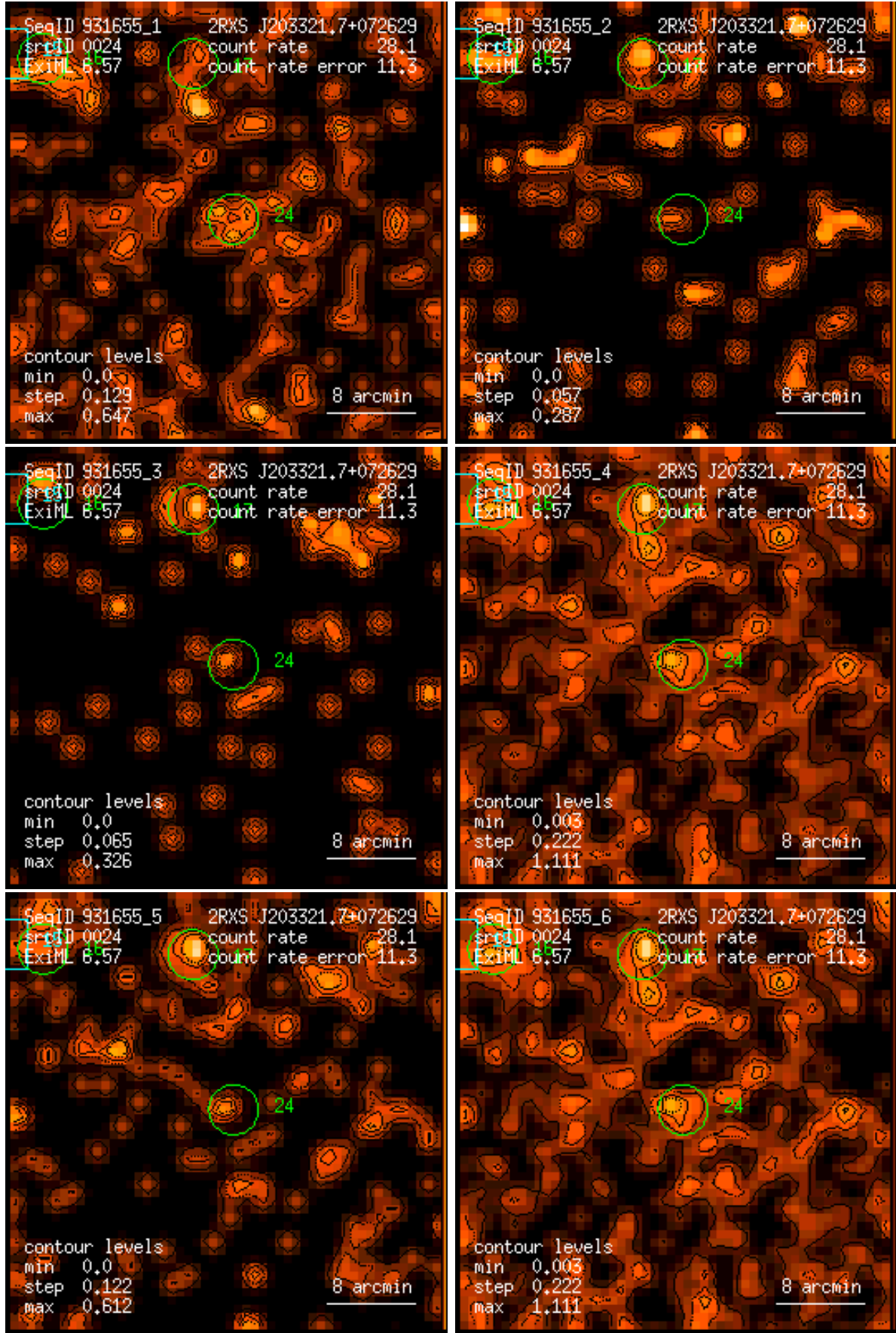
Figure 24: RASS 931655: detection 0024: band rate images, Gaussian filter: (1) PSPC channels 11 – 41, (2) 52 – 90, (3) 91 – 201, (4) 11 – 235, (5) 52 – 201, (6) 11 – 201. Broad band rates in counts/ks. Band rate contour levels in counts/ks/arcmin 2 .
