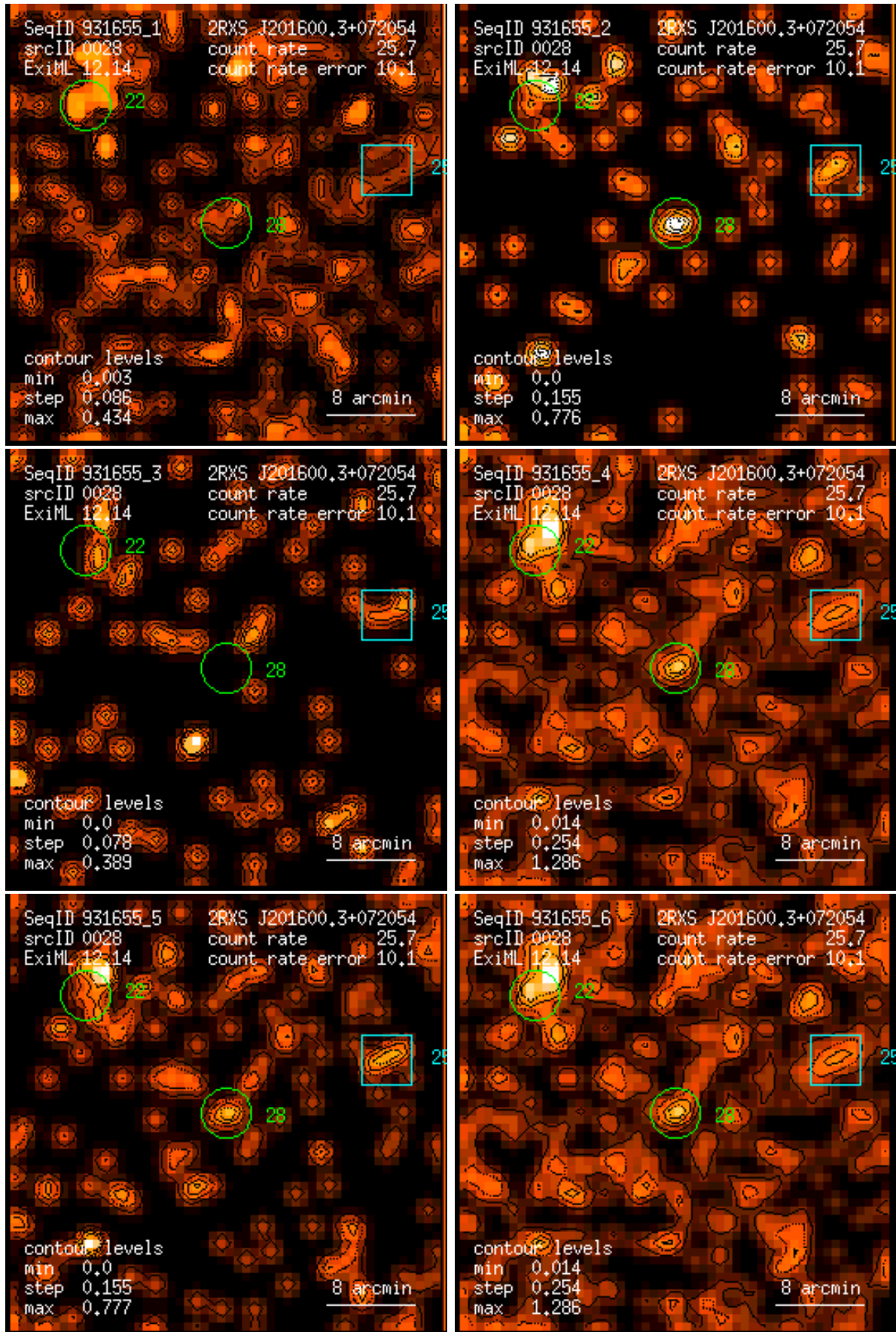
Figure 28: RASS 931655: detection 0028: band rate images, Gaussian filter: (1) PSPC channels 11 – 41, (2) 52 – 90, (3) 91 – 201, (4) 11 – 235, (5) 52 – 201, (6) 11 – 201. Broad band rates in counts/ks. Band rate contour levels in counts/ks/arcmin 2 .
