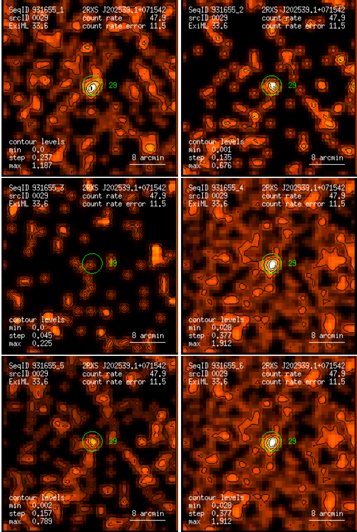
Figure 29: RASS 931655: detection 0029: band rate images, Gaussian filter: (1) PSPC channels 11 – 41, (2) 52 – 90, (3) 91 – 201, (4) 11 – 235, (5) 52 – 201, (6) 11 – 201. Broad band rates in counts/ks. Band rate contour levels in counts/ks/arcmin 2 .
