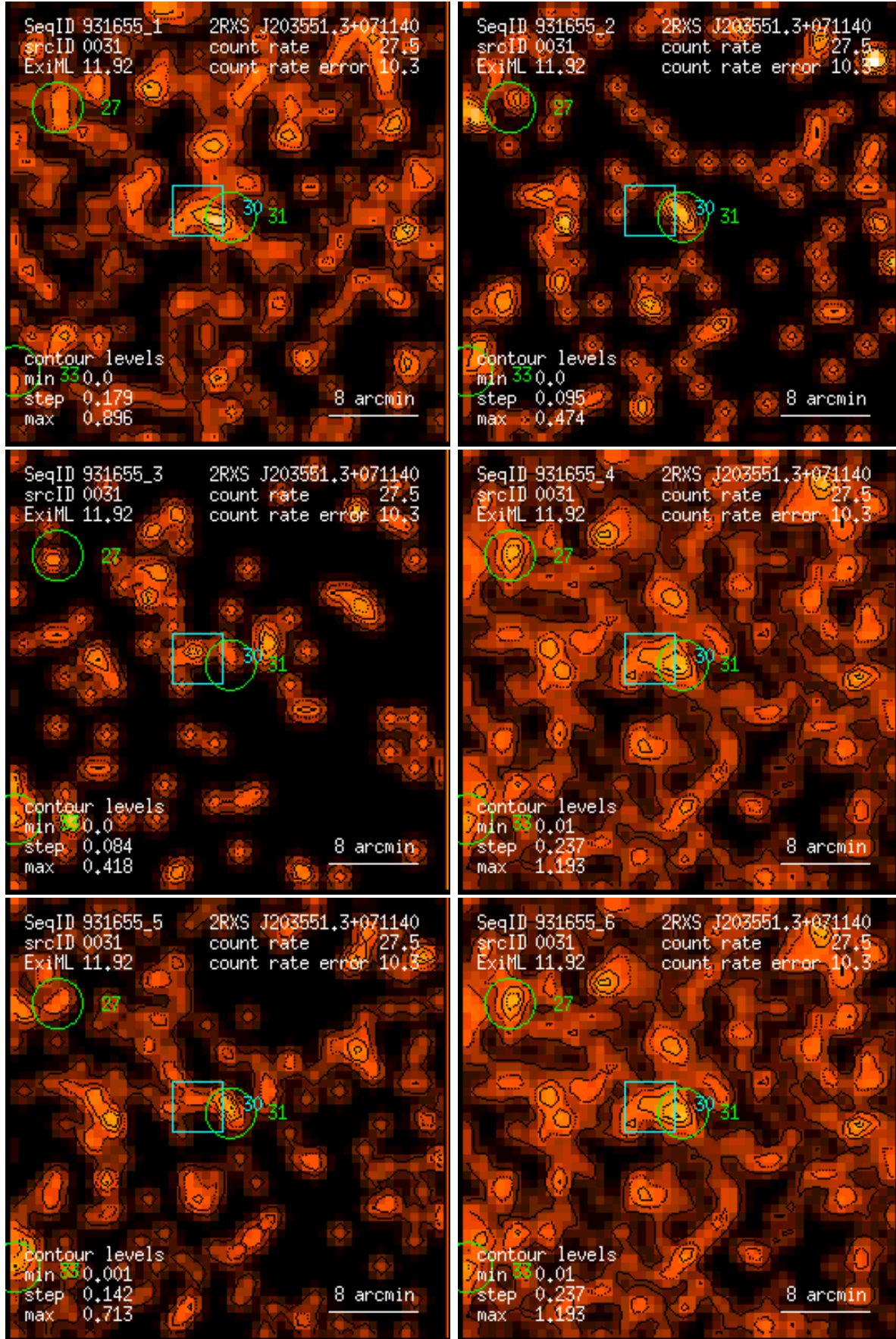
Figure 31: RASS 931655: detection 0031: band rate images, Gaussian filter: (1) PSPC channels 11 – 41, (2) 52 – 90, (3) 91 – 201, (4) 11 – 235, (5) 52 – 201, (6) 11 – 201. Broad band rates in counts/ks. Band rate contour levels in counts/ks/arcmin 2 .
