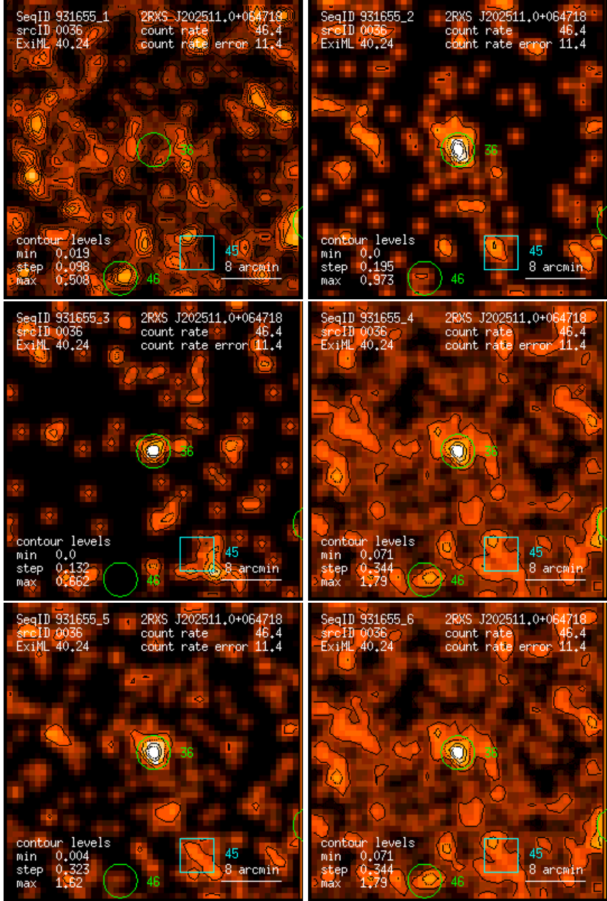
Figure 36: RASS 931655: detection 0036: band rate images, Gaussian filter: (1) PSPC channels 11 – 41, (2) 52 – 90, (3) 91 – 201, (4) 11 – 235, (5) 52 – 201, (6) 11 – 201. Broad band rates in counts/ks. Band rate contour levels in counts/ks/arcmin 2 .
