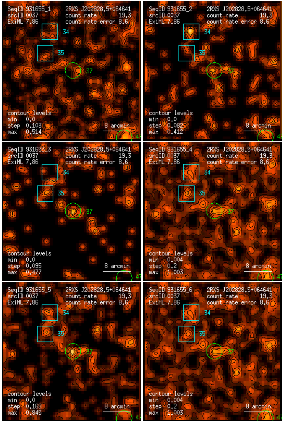
Figure 37: RASS 931655: detection 0037: band rate images, Gaussian filter: (1) PSPC channels 11 – 41, (2) 52 – 90, (3) 91 – 201, (4) 11 – 235, (5) 52 – 201, (6) 11 – 201. Broad band rates in counts/ks. Band rate contour levels in counts/ks/arcmin 2 .
