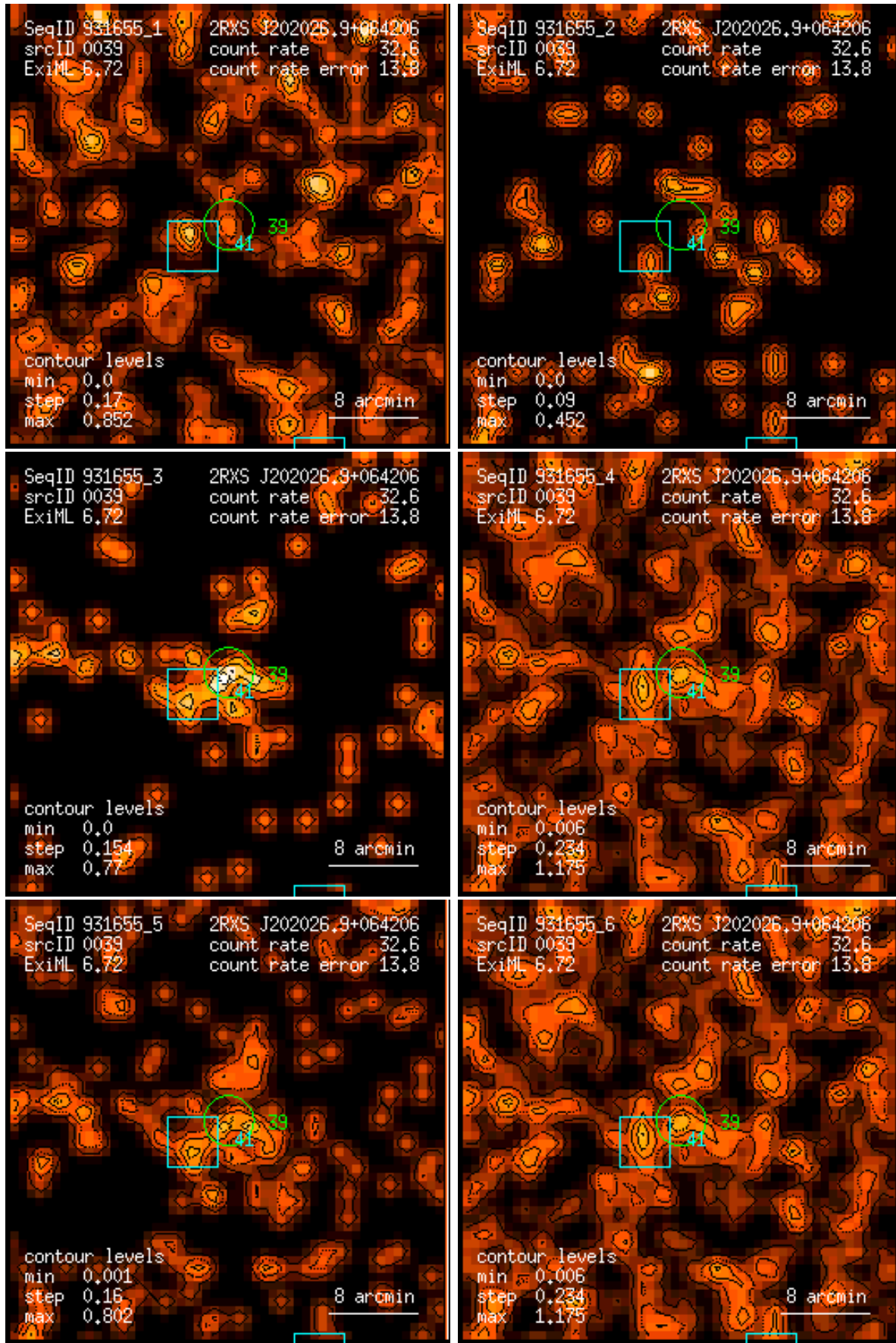
Figure 39: RASS 931655: detection 0039: band rate images, Gaussian filter: (1) PSPC channels 11 – 41, (2) 52 – 90, (3) 91 – 201, (4) 11 – 235, (5) 52 – 201, (6) 11 – 201. Broad band rates in counts/ks. Band rate contour levels in counts/ks/arcmin 2 .
