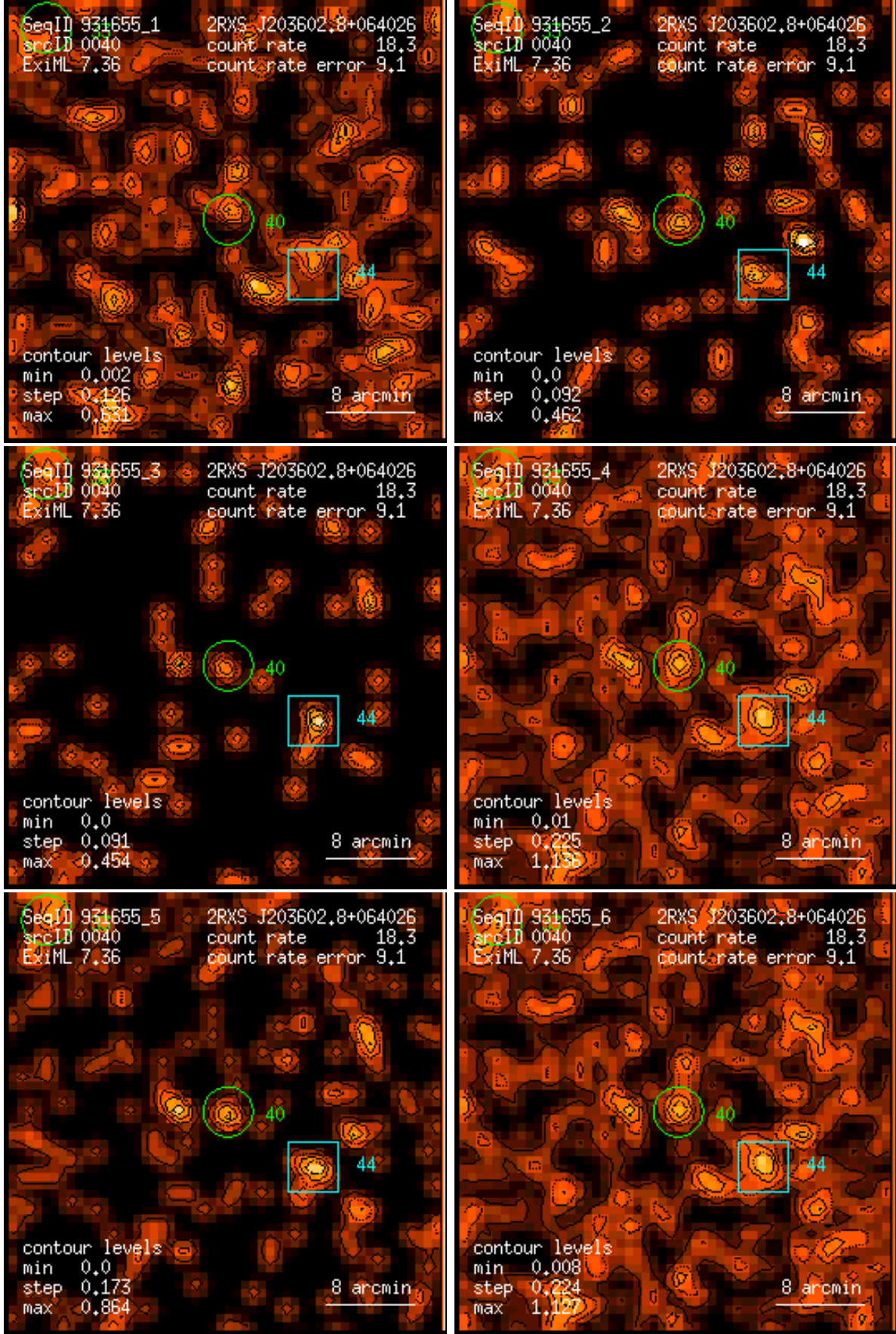
Figure 40: RASS 931655: detection 0040: band rate images, Gaussian filter: (1) PSPC channels 11 – 41, (2) 52 – 90, (3) 91 – 201, (4) 11 – 235, (5) 52 – 201, (6) 11 – 201. Broad band rates in counts/ks. Band rate contour levels in counts/ks/arcmin 2 .
