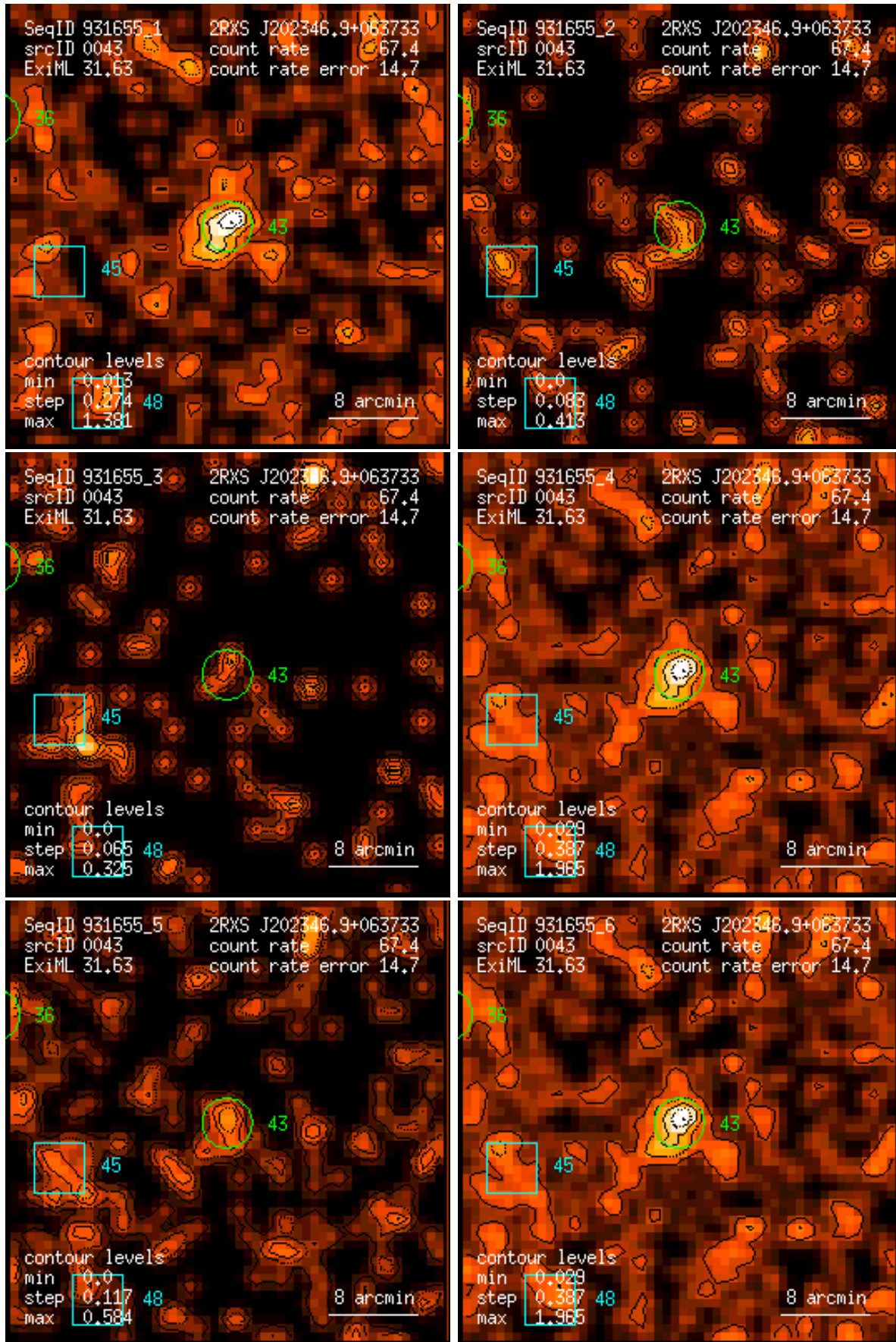
Figure 43: RASS 931655: detection 0043: band rate images, Gaussian filter: (1) PSPC channels 11 – 41, (2) 52 – 90, (3) 91 – 201, (4) 11 – 235, (5) 52 – 201, (6) 11 – 201. Broad band rates in counts/ks. Band rate contour levels in counts/ks/arcmin 2 .
