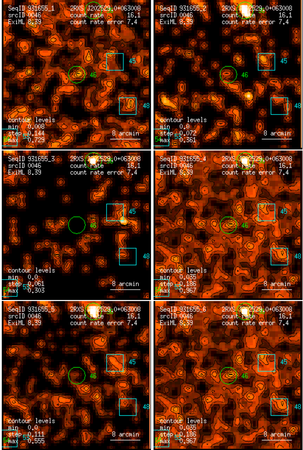
Figure 46: RASS 931655: detection 0046: band rate images, Gaussian filter: (1) PSPC channels 11 – 41, (2) 52 – 90, (3) 91 – 201, (4) 11 – 235, (5) 52 – 201, (6) 11 – 201. Broad band rates in counts/ks. Band rate contour levels in counts/ks/arcmin 2 .
