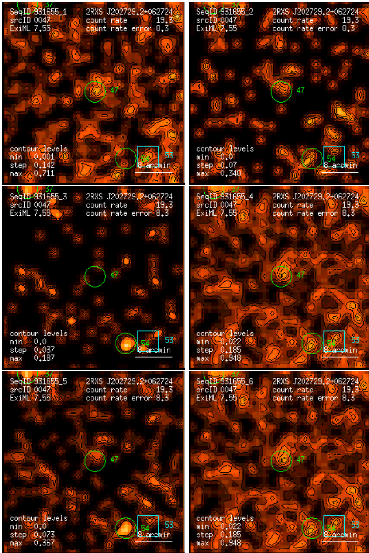
Figure 47: RASS 931655: detection 0047: band rate images, Gaussian filter: (1) PSPC channels 11 – 41, (2) 52 – 90, (3) 91 – 201, (4) 11 – 235, (5) 52 – 201, (6) 11 – 201. Broad band rates in counts/ks. Band rate contour levels in counts/ks/arcmin 2 .
