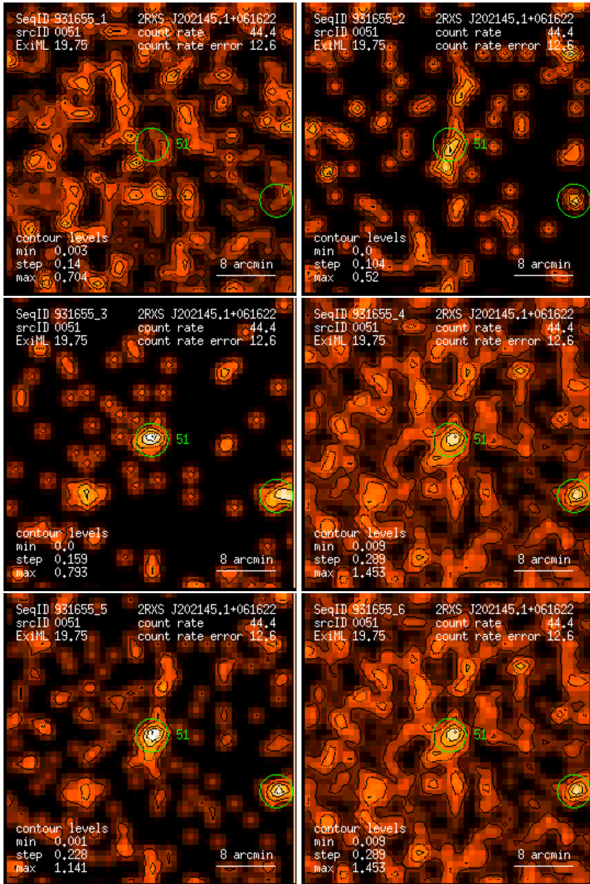
Figure 51: RASS 931655: detection 0051: band rate images, Gaussian filter: (1) PSPC channels 11 – 41, (2) 52 – 90, (3) 91 – 201, (4) 11 – 235, (5) 52 – 201, (6) 11 – 201. Broad band rates in counts/ks. Band rate contour levels in counts/ks/arcmin 2 .
