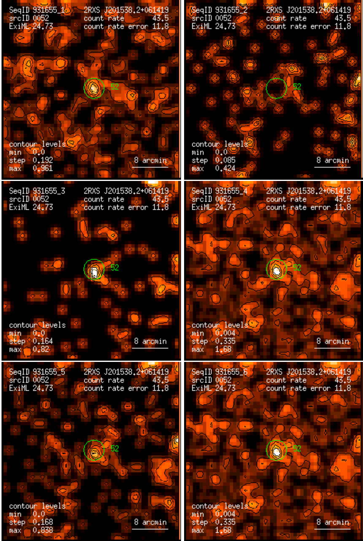
Figure 52: RASS 931655: detection 0052: band rate images, Gaussian filter: (1) PSPC channels 11 – 41, (2) 52 – 90, (3) 91 – 201, (4) 11 – 235, (5) 52 – 201, (6) 11 – 201. Broad band rates in counts/ks. Band rate contour levels in counts/ks/arcmin 2 .
