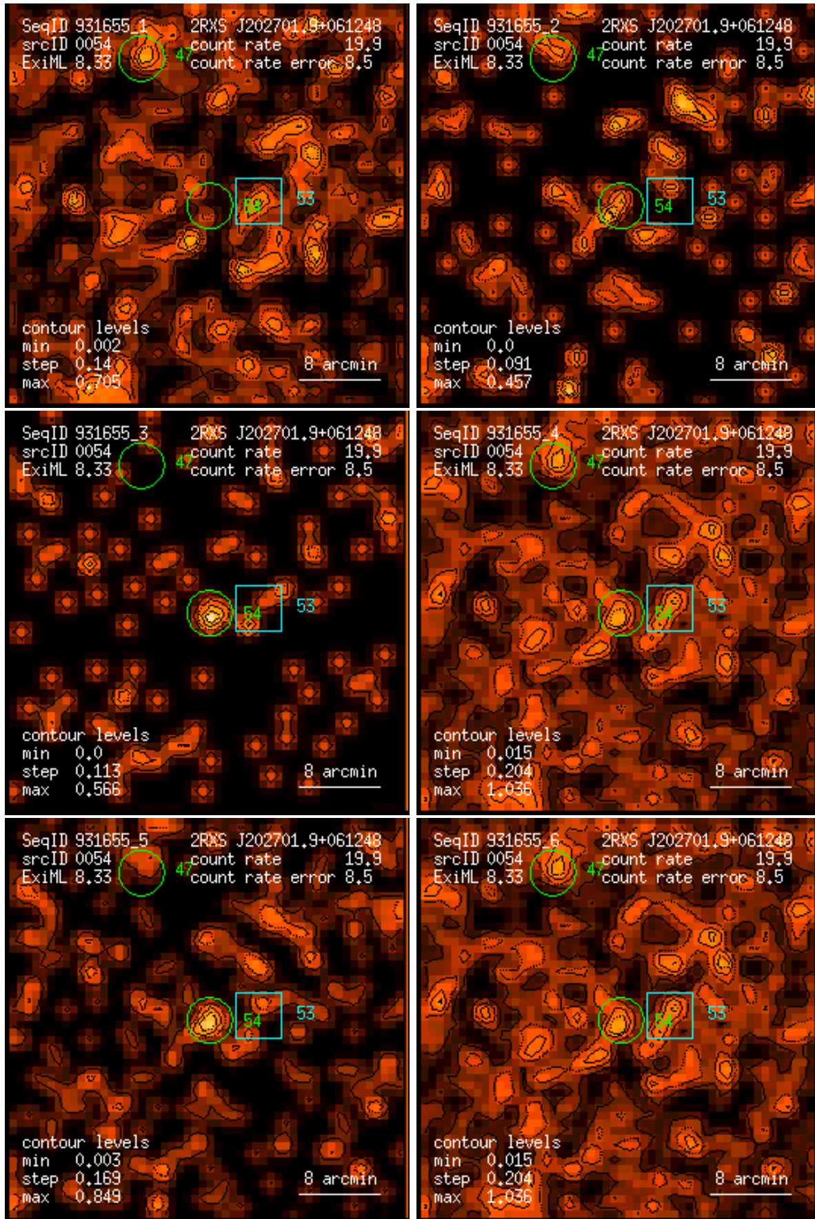
Figure 54: RASS 931655: detection 0054: band rate images, Gaussian filter: (1) PSPC channels 11 – 41, (2) 52 – 90, (3) 91 – 201, (4) 11 – 235, (5) 52 – 201, (6) 11 – 201. Broad band rates in counts/ks. Band rate contour levels in counts/ks/arcmin 2 .
