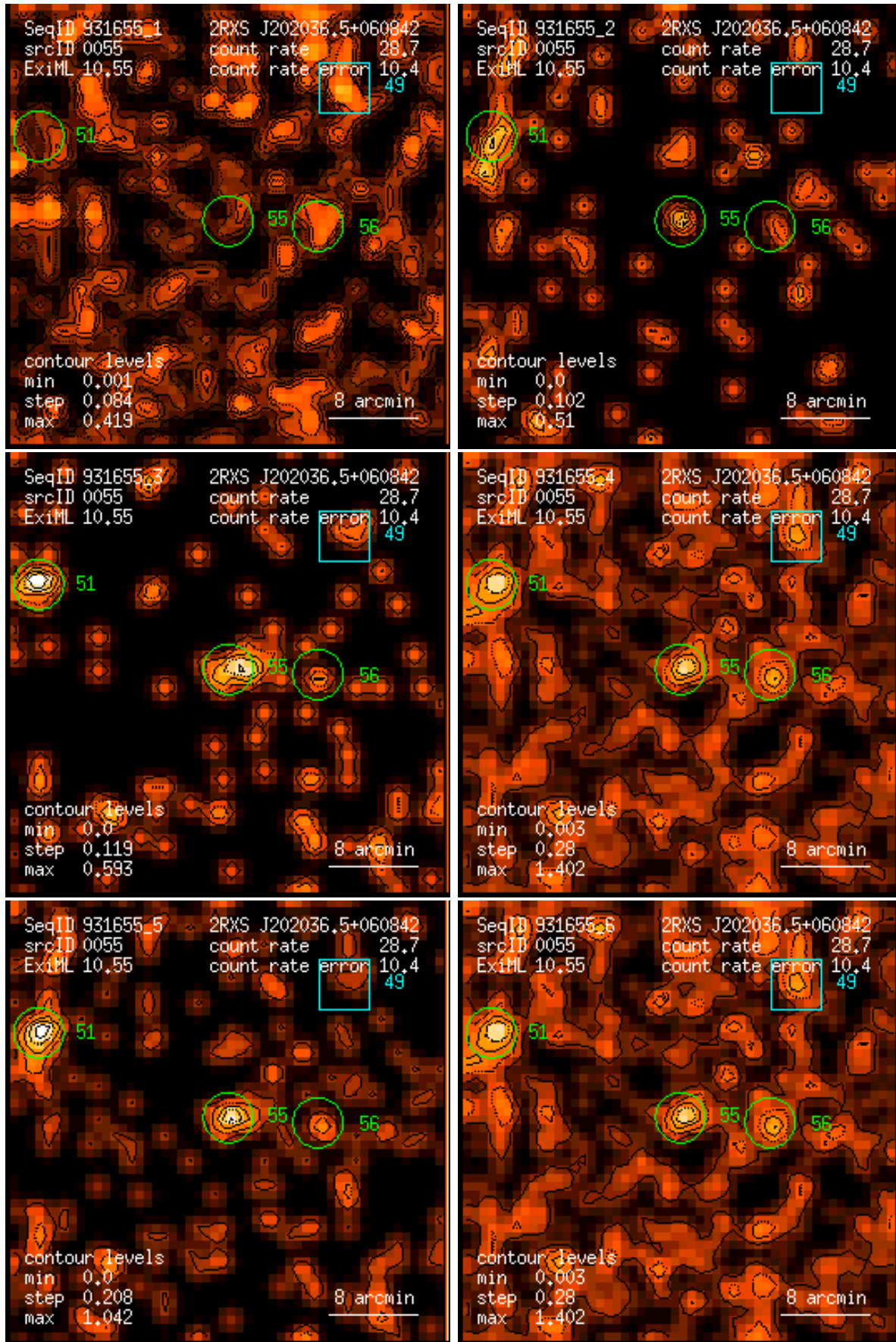
Figure 55: RASS 931655: detection 0055: band rate images, Gaussian filter: (1) PSPC channels 11 – 41, (2) 52 – 90, (3) 91 – 201, (4) 11 – 235, (5) 52 – 201, (6) 11 – 201. Broad band rates in counts/ks. Band rate contour levels in counts/ks/arcmin 2 .
