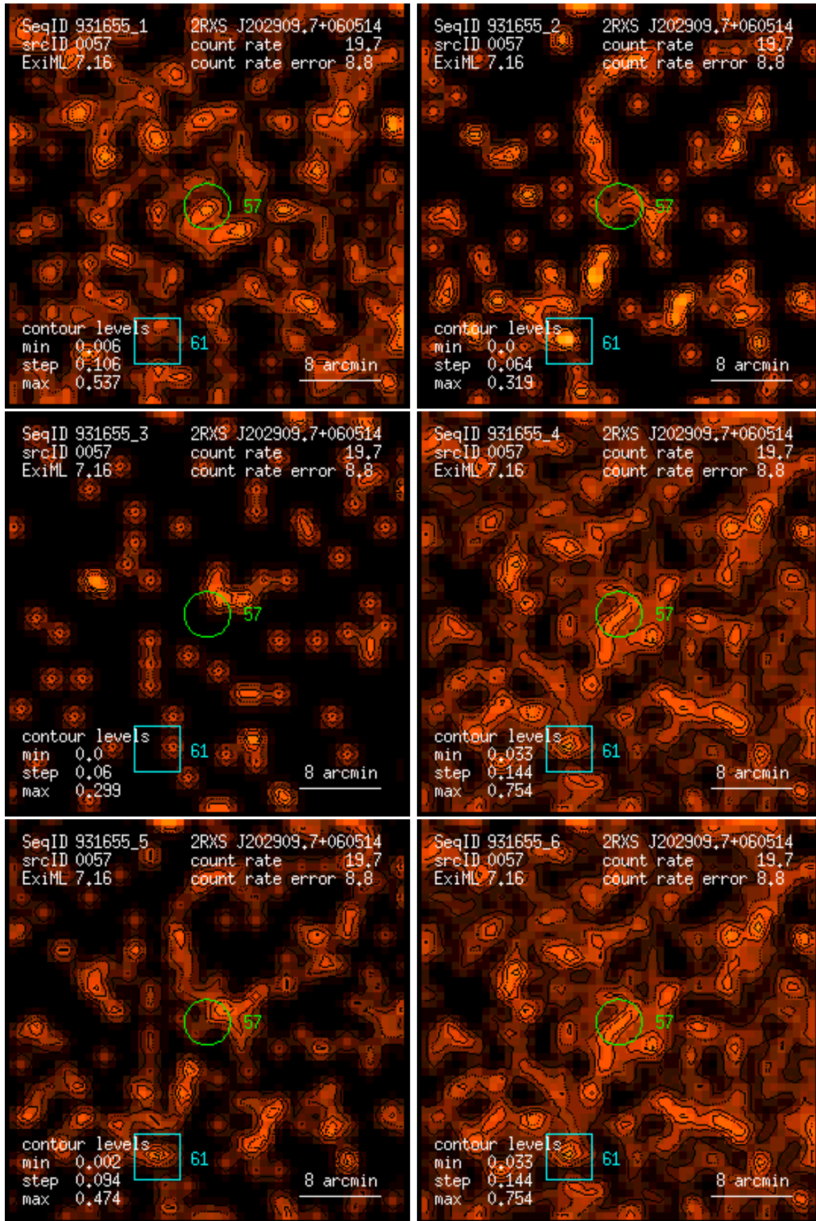
Figure 57: RASS 931655: detection 0057: band rate images, Gaussian filter: (1) PSPC channels 11 – 41, (2) 52 – 90, (3) 91 – 201, (4) 11 – 235, (5) 52 – 201, (6) 11 – 201. Broad band rates in counts/ks. Band rate contour levels in counts/ks/arcmin 2 .
