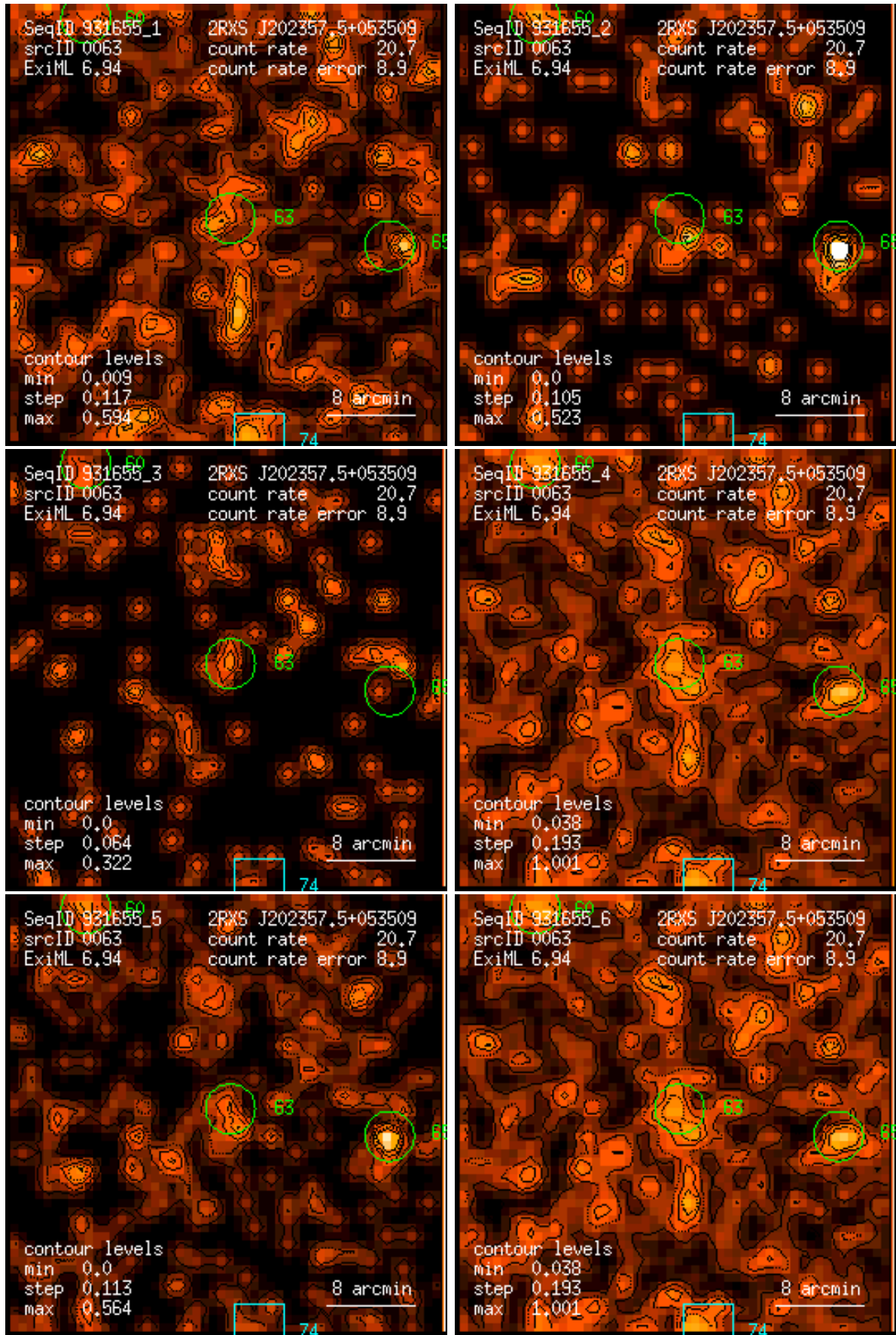
Figure 63: RASS 931655: detection 0063: band rate images, Gaussian filter: (1) PSPC channels 11 – 41, (2) 52 – 90, (3) 91 – 201, (4) 11 – 235, (5) 52 – 201, (6) 11 – 201. Broad band rates in counts/ks. Band rate contour levels in counts/ks/arcmin 2 .
