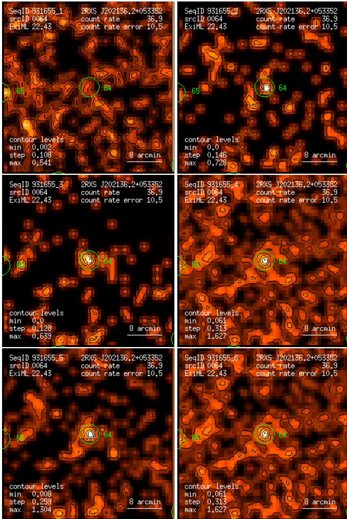
Figure 64: RASS 931655: detection 0064: band rate images, Gaussian filter: (1) PSPC channels 11 – 41, (2) 52 – 90, (3) 91 – 201, (4) 11 – 235, (5) 52 – 201, (6) 11 – 201. Broad band rates in counts/ks. Band rate contour levels in counts/ks/arcmin 2 .
