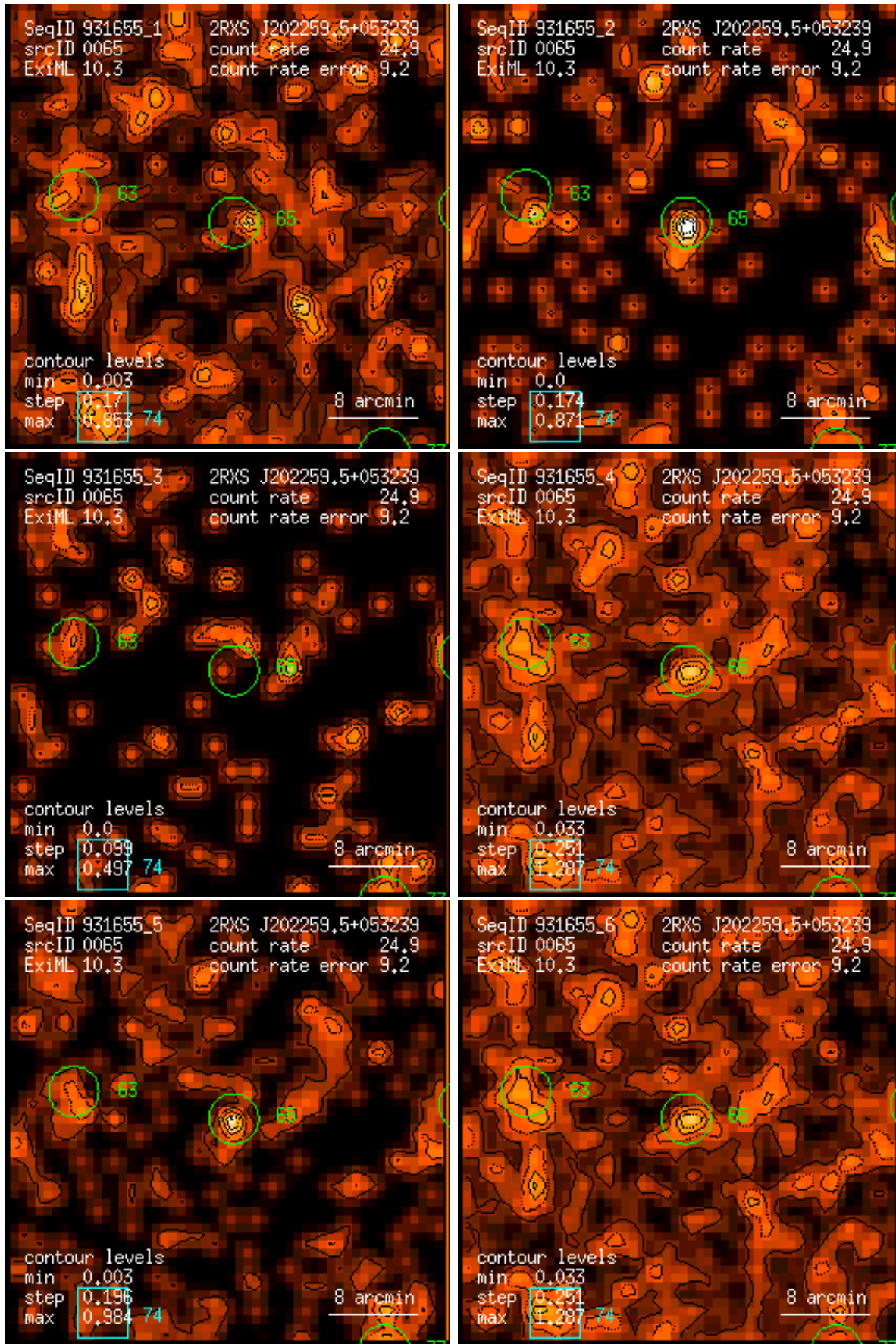
Figure 65: RASS 931655: detection 0065: band rate images, Gaussian filter: (1) PSPC channels 11 – 41, (2) 52 – 90, (3) 91 – 201, (4) 11 – 235, (5) 52 – 201, (6) 11 – 201. Broad band rates in counts/ks. Band rate contour levels in counts/ks/arcmin 2 .
