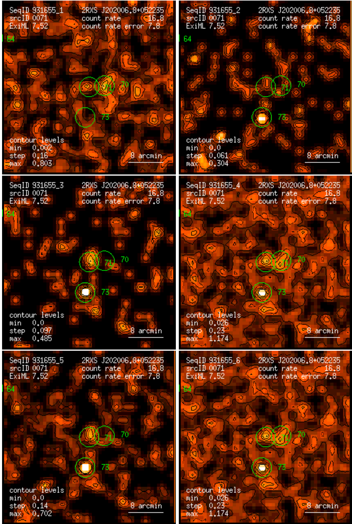
Figure 71: RASS 931655: detection 0071: band rate images, Gaussian filter: (1) PSPC channels 11 – 41, (2) 52 – 90, (3) 91 – 201, (4) 11 – 235, (5) 52 – 201, (6) 11 – 201. Broad band rates in counts/ks. Band rate contour levels in counts/ks/arcmin 2 .
