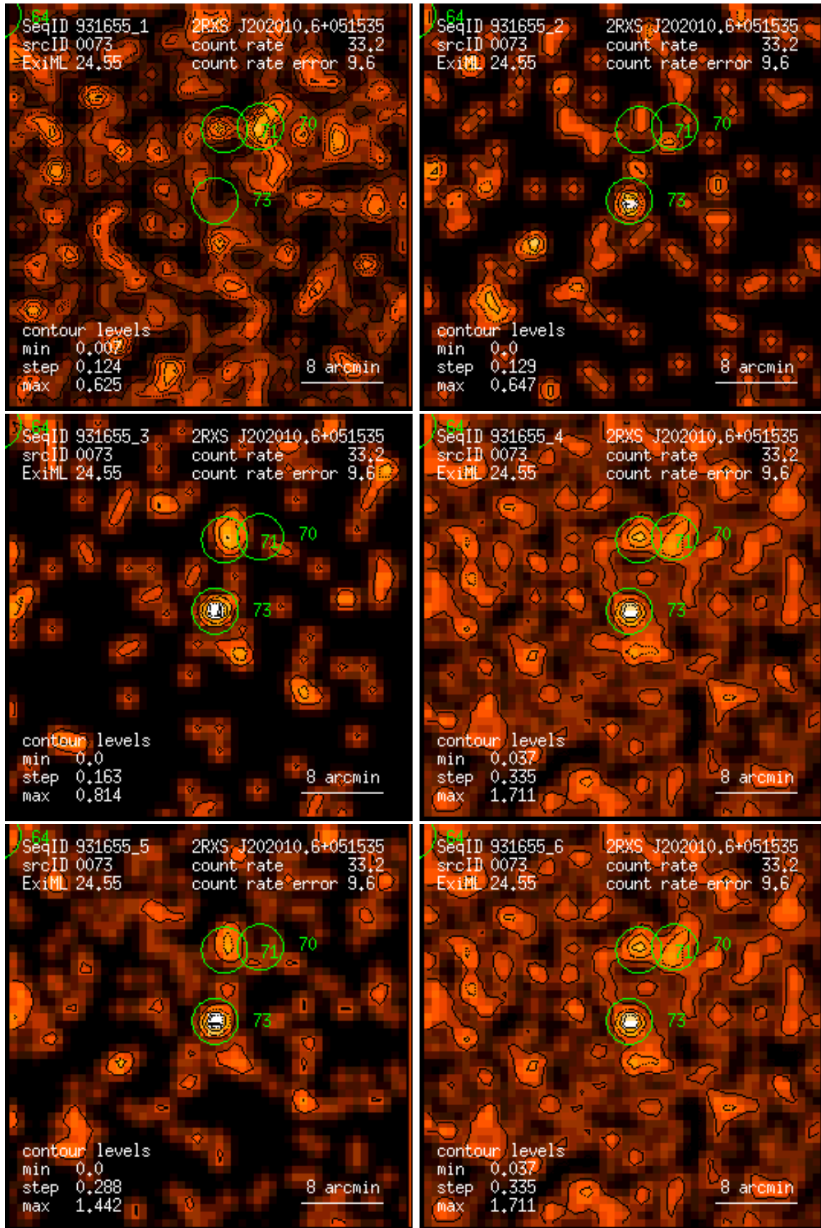
Figure 73: RASS 931655: detection 0073: band rate images, Gaussian filter: (1) PSPC channels 11 – 41, (2) 52 – 90, (3) 91 – 201, (4) 11 – 235, (5) 52 – 201, (6) 11 – 201. Broad band rates in counts/ks. Band rate contour levels in counts/ks/arcmin 2 .
