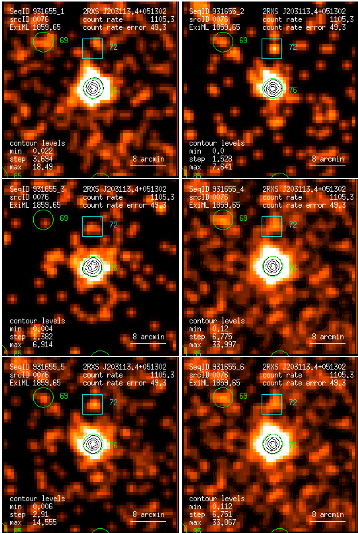
Figure 76: RASS 931655: detection 0076: band rate images, Gaussian filter: (1) PSPC channels 11 – 41, (2) 52 – 90, (3) 91 – 201, (4) 11 – 235, (5) 52 – 201, (6) 11 – 201. Broad band rates in counts/ks. Band rate contour levels in counts/ks/arcmin 2 .
