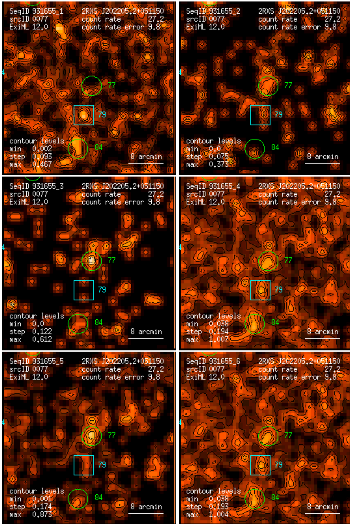
Figure 77: RASS 931655: detection 0077: band rate images, Gaussian filter: (1) PSPC channels 11 – 41, (2) 52 – 90, (3) 91 – 201, (4) 11 – 235, (5) 52 – 201, (6) 11 – 201. Broad band rates in counts/ks. Band rate contour levels in counts/ks/arcmin 2 .
