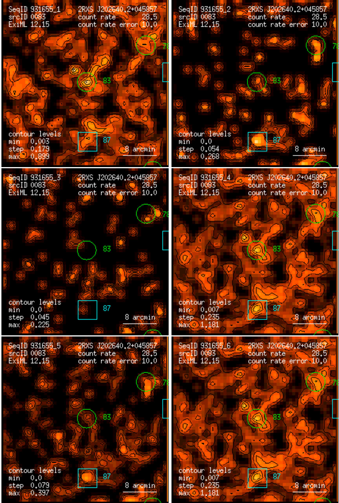
Figure 83: RASS 931655: detection 0083: band rate images, Gaussian filter: (1) PSPC channels 11 – 41, (2) 52 – 90, (3) 91 – 201, (4) 11 – 235, (5) 52 – 201, (6) 11 – 201. Broad band rates in counts/ks. Band rate contour levels in counts/ks/arcmin 2 .
