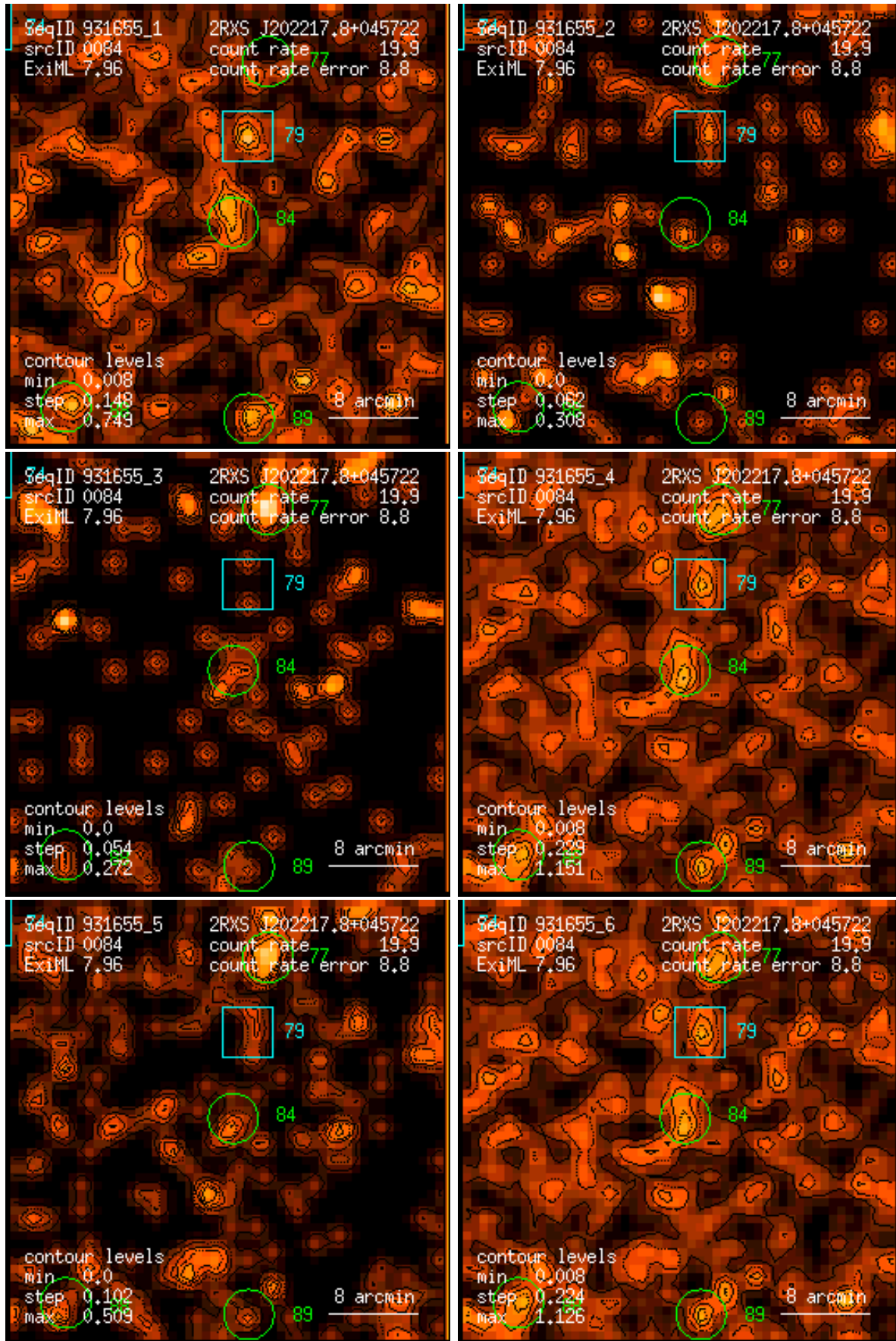
Figure 84: RASS 931655: detection 0084: band rate images, Gaussian filter: (1) PSPC channels 11 – 41, (2) 52 – 90, (3) 91 – 201, (4) 11 – 235, (5) 52 – 201, (6) 11 – 201. Broad band rates in counts/ks. Band rate contour levels in counts/ks/arcmin 2 .
