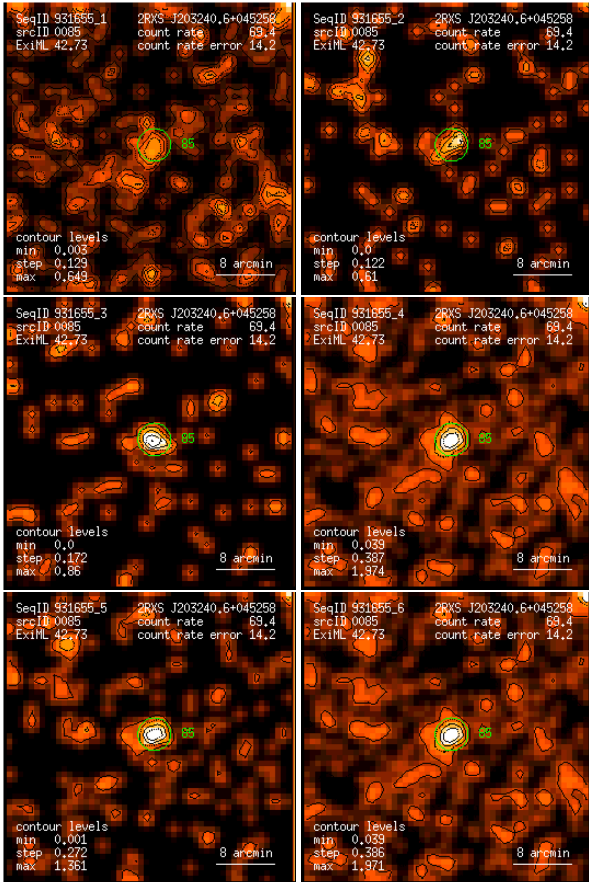
Figure 85: RASS 931655: detection 0085: band rate images, Gaussian filter: (1) PSPC channels 11 – 41, (2) 52 – 90, (3) 91 – 201, (4) 11 – 235, (5) 52 – 201, (6) 11 – 201. Broad band rates in counts/ks. Band rate contour levels in counts/ks/arcmin 2 .
