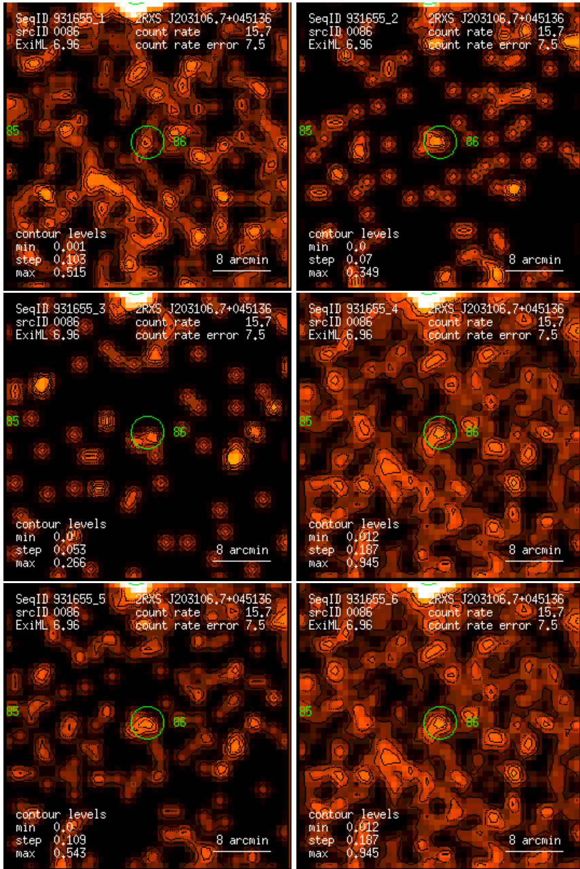
Figure 86: RASS 931655: detection 0086: band rate images, Gaussian filter: (1) PSPC channels 11 – 41, (2) 52 – 90, (3) 91 – 201, (4) 11 – 235, (5) 52 – 201, (6) 11 – 201. Broad band rates in counts/ks. Band rate contour levels in counts/ks/arcmin 2 .
