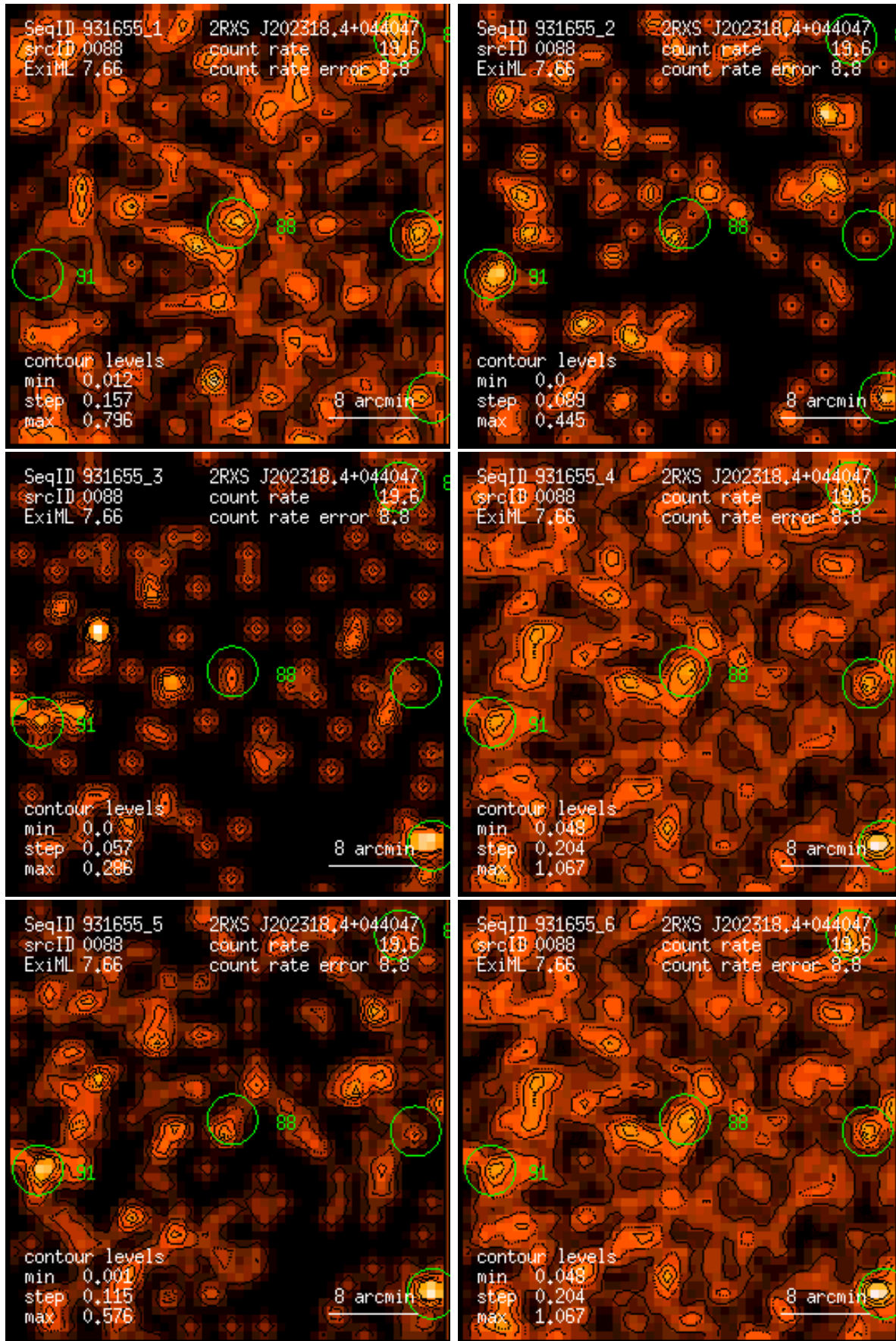
Figure 88: RASS 931655: detection 0088: band rate images, Gaussian filter: (1) PSPC channels 11 – 41, (2) 52 – 90, (3) 91 – 201, (4) 11 – 235, (5) 52 – 201, (6) 11 – 201. Broad band rates in counts/ks. Band rate contour levels in counts/ks/arcmin 2 .
