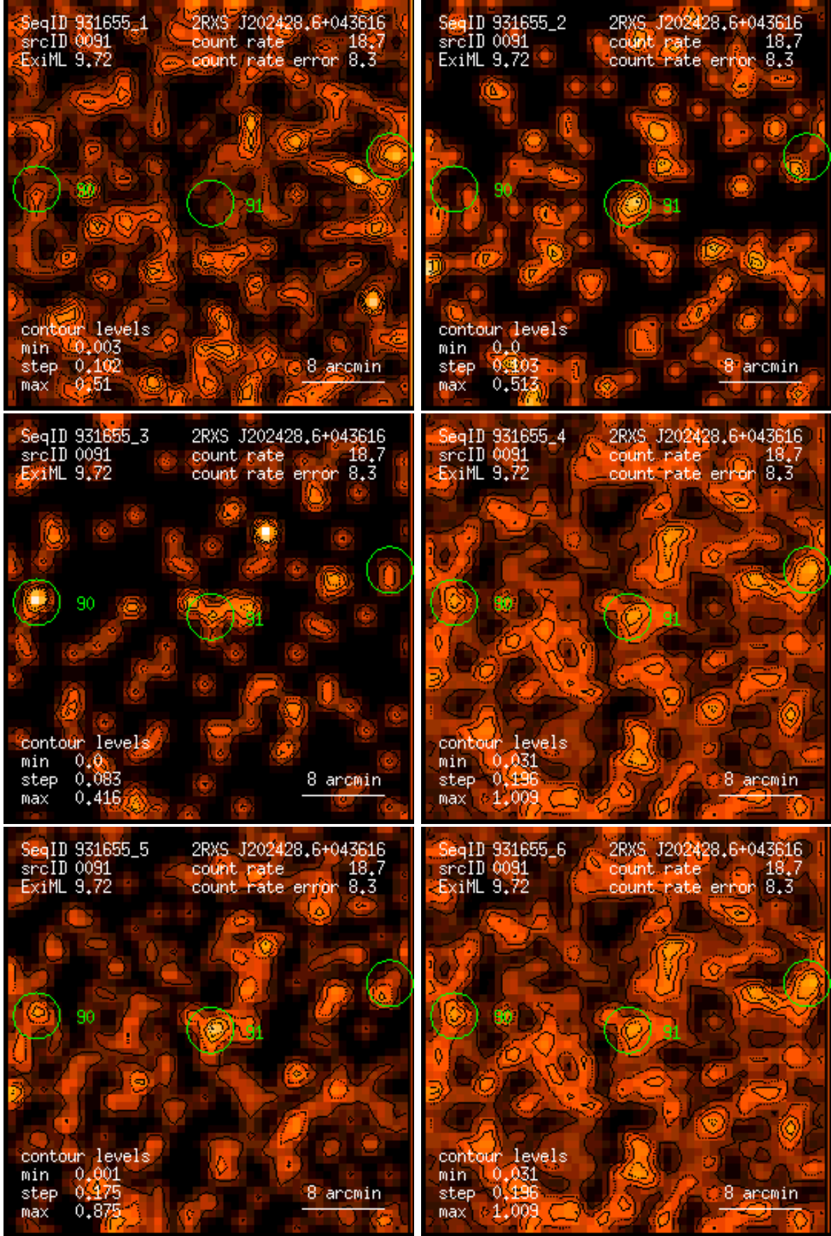
Figure 91: RASS 931655: detection 0091: band rate images, Gaussian filter: (1) PSPC channels 11 – 41, (2) 52 – 90, (3) 91 – 201, (4) 11 – 235, (5) 52 – 201, (6) 11 – 201. Broad band rates in counts/ks. Band rate contour levels in counts/ks/arcmin 2 .
