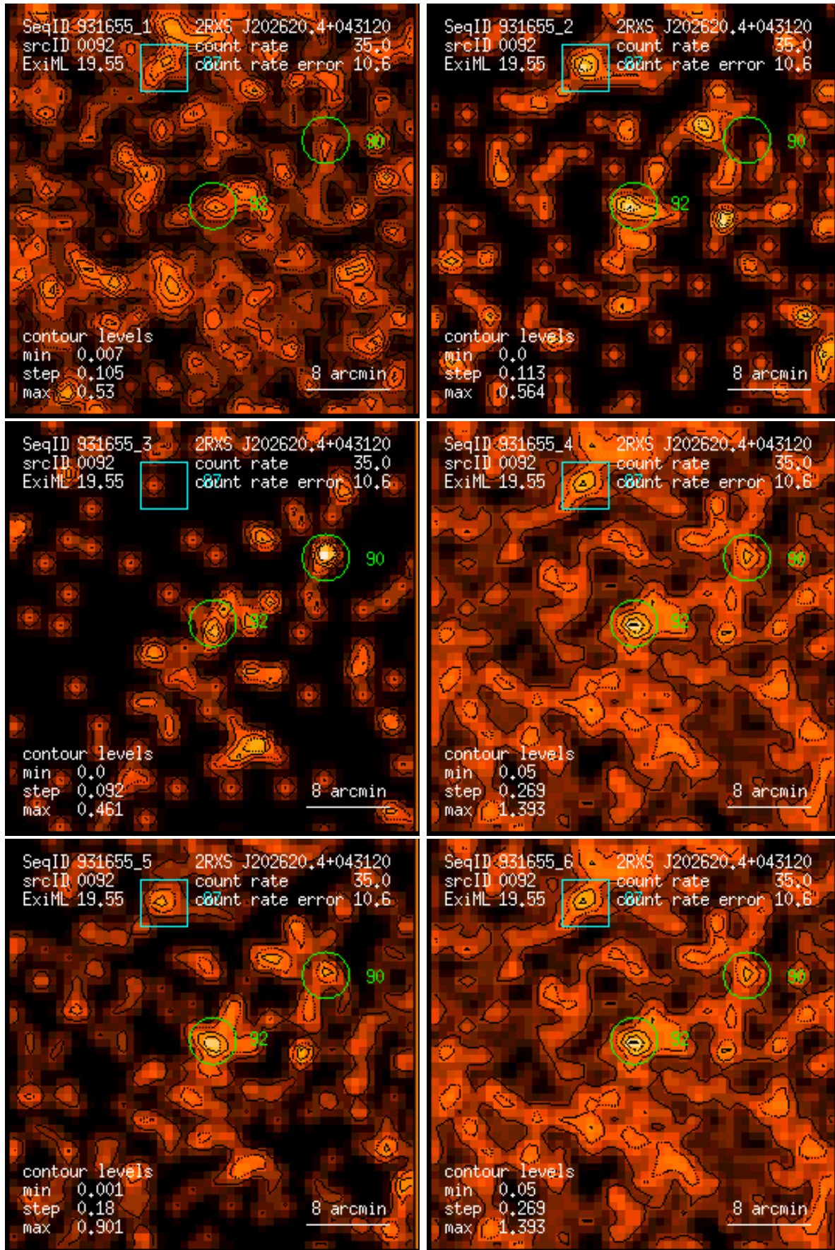
Figure 92: RASS 931655: detection 0092: band rate images, Gaussian filter: (1) PSPC channels 11 – 41, (2) 52 – 90, (3) 91 – 201, (4) 11 – 235, (5) 52 – 201, (6) 11 – 201. Broad band rates in counts/ks. Band rate contour levels in counts/ks/arcmin 2 .
