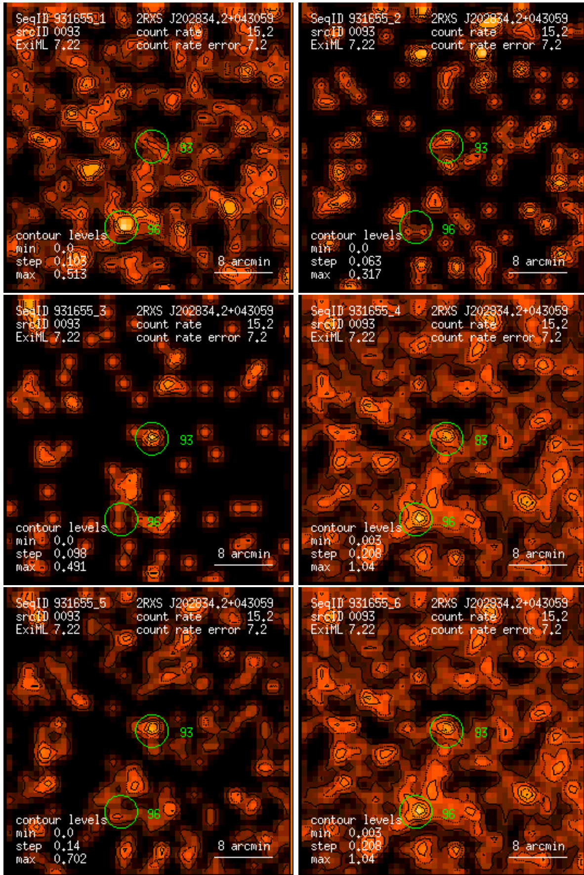
Figure 93: RASS 931655: detection 0093: band rate images, Gaussian filter: (1) PSPC channels 11 – 41, (2) 52 – 90, (3) 91 – 201, (4) 11 – 235, (5) 52 – 201, (6) 11 – 201. Broad band rates in counts/ks. Band rate contour levels in counts/ks/arcmin 2 .
