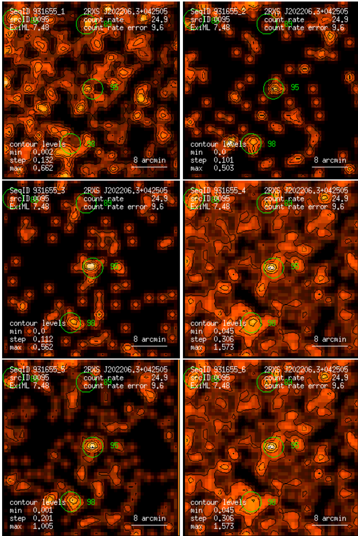
Figure 95: RASS 931655: detection 0095: band rate images, Gaussian filter: (1) PSPC channels 11 – 41, (2) 52 – 90, (3) 91 – 201, (4) 11 – 235, (5) 52 – 201, (6) 11 – 201. Broad band rates in counts/ks. Band rate contour levels in counts/ks/arcmin 2 .
