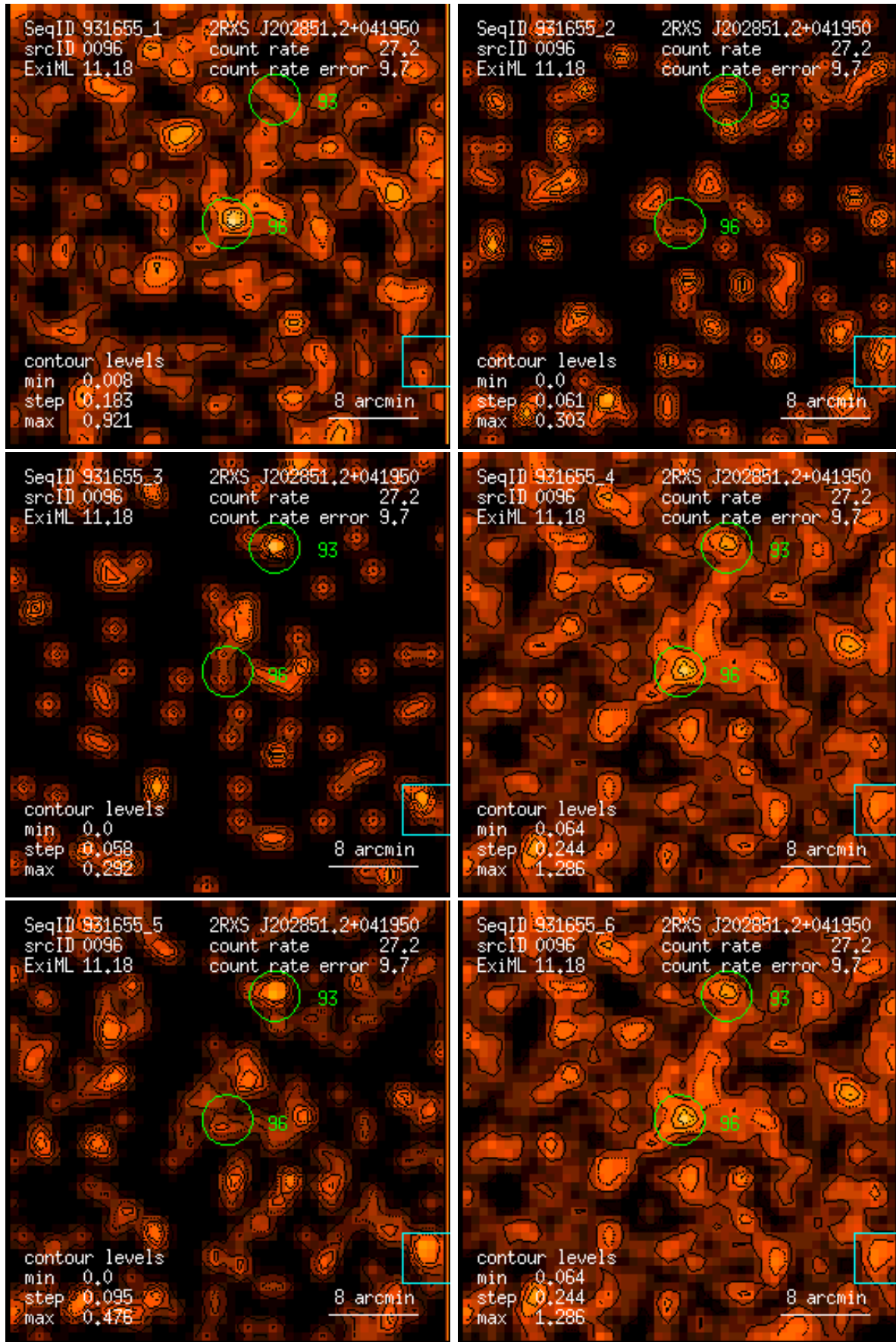
Figure 96: RASS 931655: detection 0096: band rate images, Gaussian filter: (1) PSPC channels 11 – 41, (2) 52 – 90, (3) 91 – 201, (4) 11 – 235, (5) 52 – 201, (6) 11 – 201. Broad band rates in counts/ks. Band rate contour levels in counts/ks/arcmin 2 .
