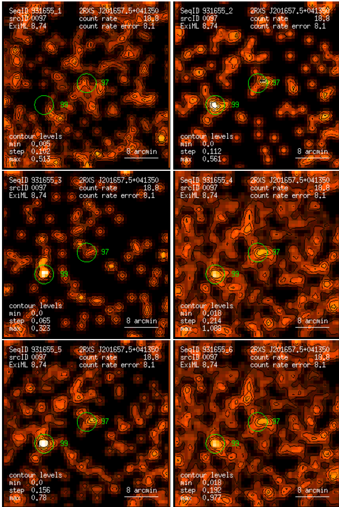
Figure 97: RASS 931655: detection 0097: band rate images, Gaussian filter: (1) PSPC channels 11 – 41, (2) 52 – 90, (3) 91 – 201, (4) 11 – 235, (5) 52 – 201, (6) 11 – 201. Broad band rates in counts/ks. Band rate contour levels in counts/ks/arcmin 2 .
