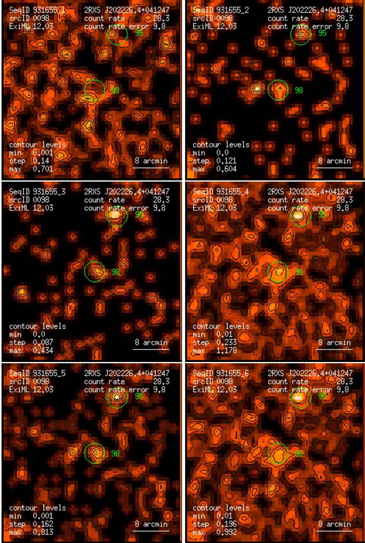
Figure 98: RASS 931655: detection 0098: band rate images, Gaussian filter: (1) PSPC channels 11 – 41, (2) 52 – 90, (3) 91 – 201, (4) 11 – 235, (5) 52 – 201, (6) 11 – 201. Broad band rates in counts/ks. Band rate contour levels in counts/ks/arcmin 2 .
