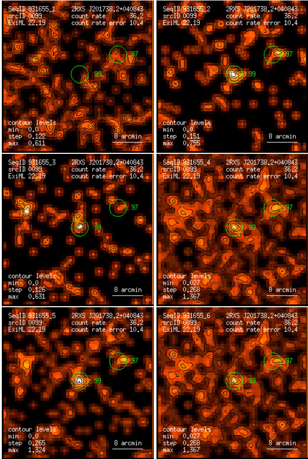
Figure 99: RASS 931655: detection 0099: band rate images, Gaussian filter: (1) PSPC channels 11 – 41, (2) 52 – 90, (3) 91 – 201, (4) 11 – 235, (5) 52 – 201, (6) 11 – 201. Broad band rates in counts/ks. Band rate contour levels in counts/ks/arcmin 2 .
