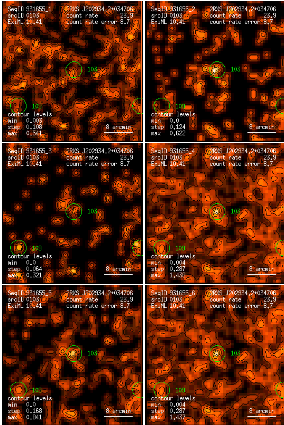
Figure 103: RASS 931655: detection 0103: band rate images, Gaussian filter: (1) PSPC channels 11 – 41, (2) 52 – 90, (3) 91 – 201, (4) 11 – 235, (5) 52 – 201, (6) 11 – 201. Broad band rates in counts/ks. Band rate contour levels in counts/ks/arcmin 2 .
