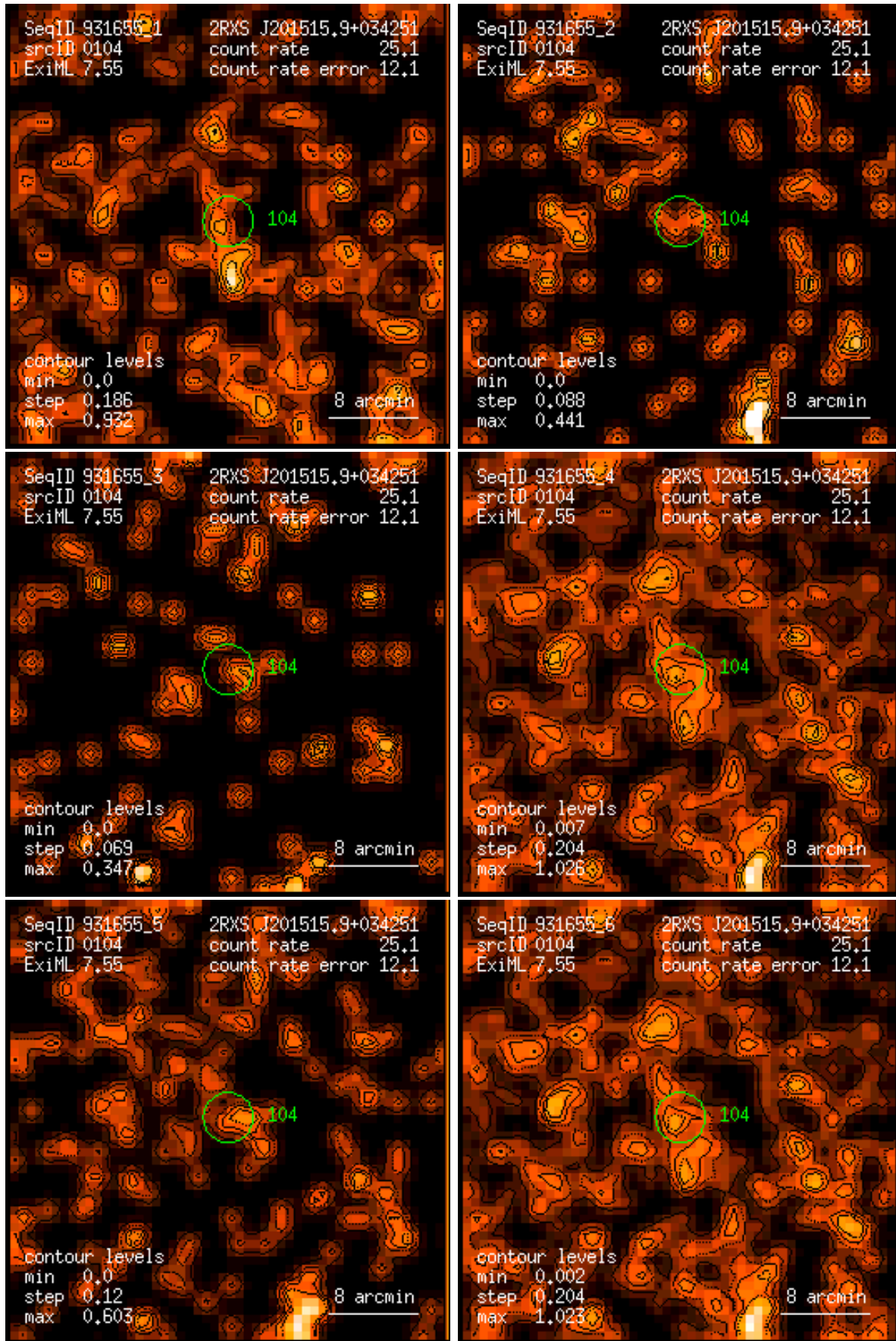
Figure 104: RASS 931655: detection 0104: band rate images, Gaussian filter: (1) PSPC channels 11 – 41, (2) 52 – 90, (3) 91 – 201, (4) 11 – 235, (5) 52 – 201, (6) 11 – 201. Broad band rates in counts/ks. Band rate contour levels in counts/ks/arcmin 2 .
