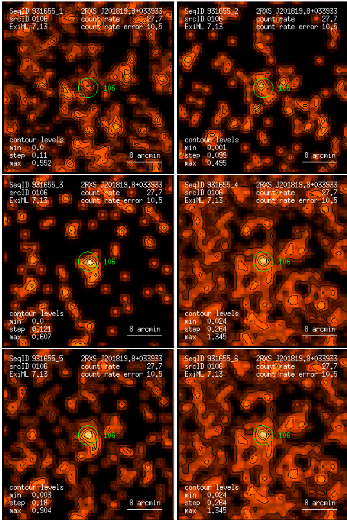
Figure 106: RASS 931655: detection 0106: band rate images, Gaussian filter: (1) PSPC channels 11 – 41, (2) 52 – 90, (3) 91 – 201, (4) 11 – 235, (5) 52 – 201, (6) 11 – 201. Broad band rates in counts/ks. Band rate contour levels in counts/ks/arcmin 2 .
