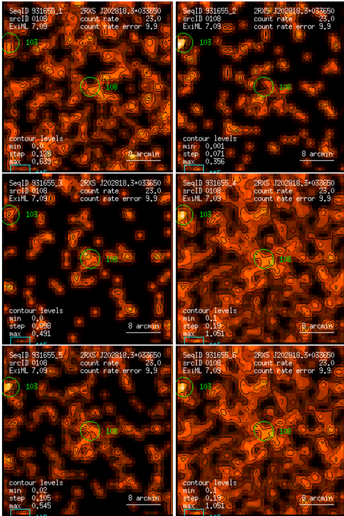
Figure 108: RASS 931655: detection 0108: band rate images, Gaussian filter: (1) PSPC channels 11 – 41, (2) 52 – 90, (3) 91 – 201, (4) 11 – 235, (5) 52 – 201, (6) 11 – 201. Broad band rates in counts/ks. Band rate contour levels in counts/ks/arcmin 2 .
