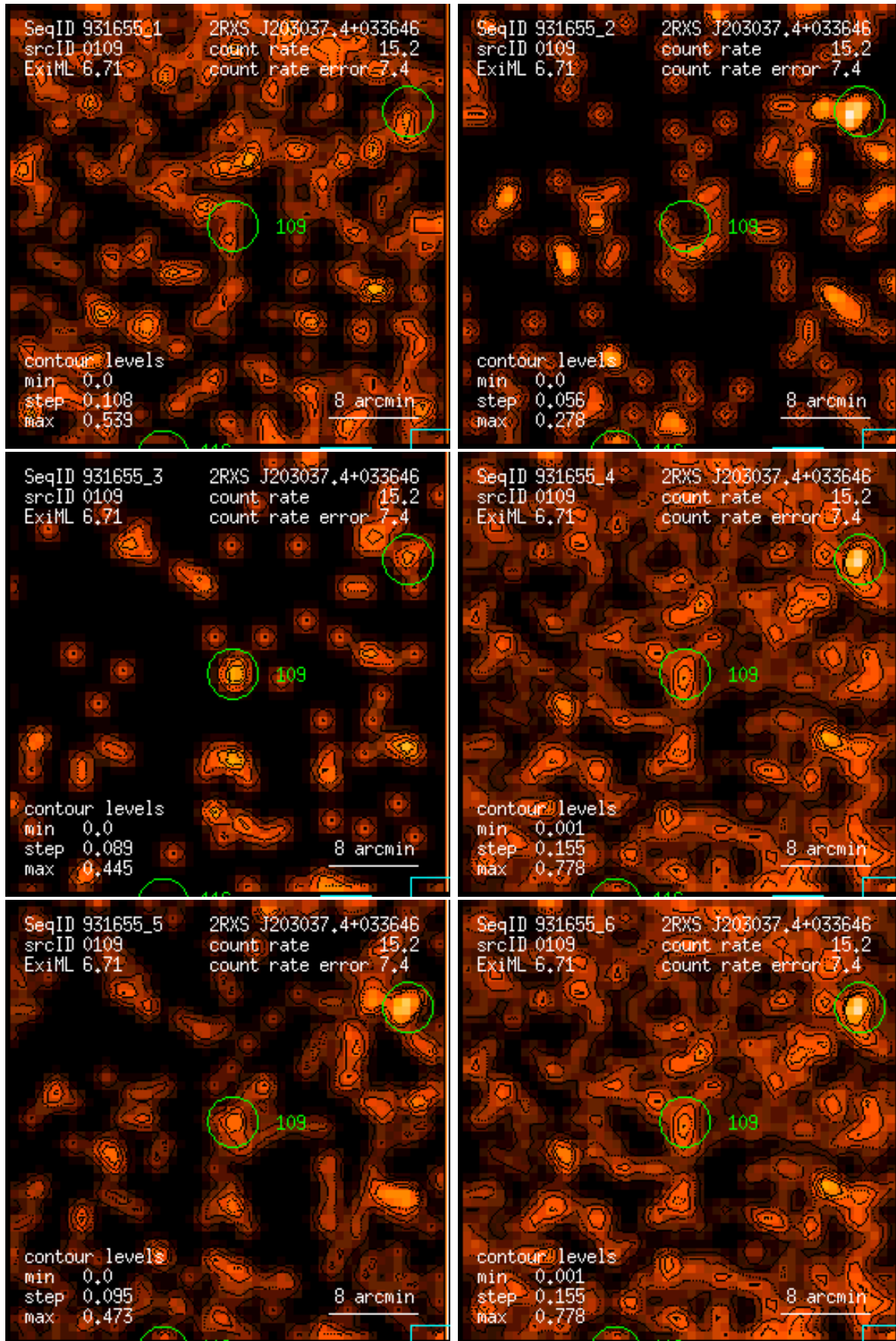
Figure 109: RASS 931655: detection 0109: band rate images, Gaussian filter: (1) PSPC channels 11 – 41, (2) 52 – 90, (3) 91 – 201, (4) 11 – 235, (5) 52 – 201, (6) 11 – 201. Broad band rates in counts/ks. Band rate contour levels in counts/ks/arcmin 2 .
