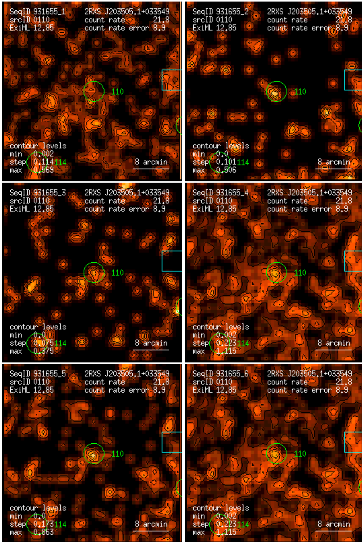
Figure 110: RASS 931655: detection 0110: band rate images, Gaussian filter: (1) PSPC channels 11 – 41, (2) 52 – 90, (3) 91 – 201, (4) 11 – 235, (5) 52 – 201, (6) 11 – 201. Broad band rates in counts/ks. Band rate contour levels in counts/ks/arcmin 2 .
