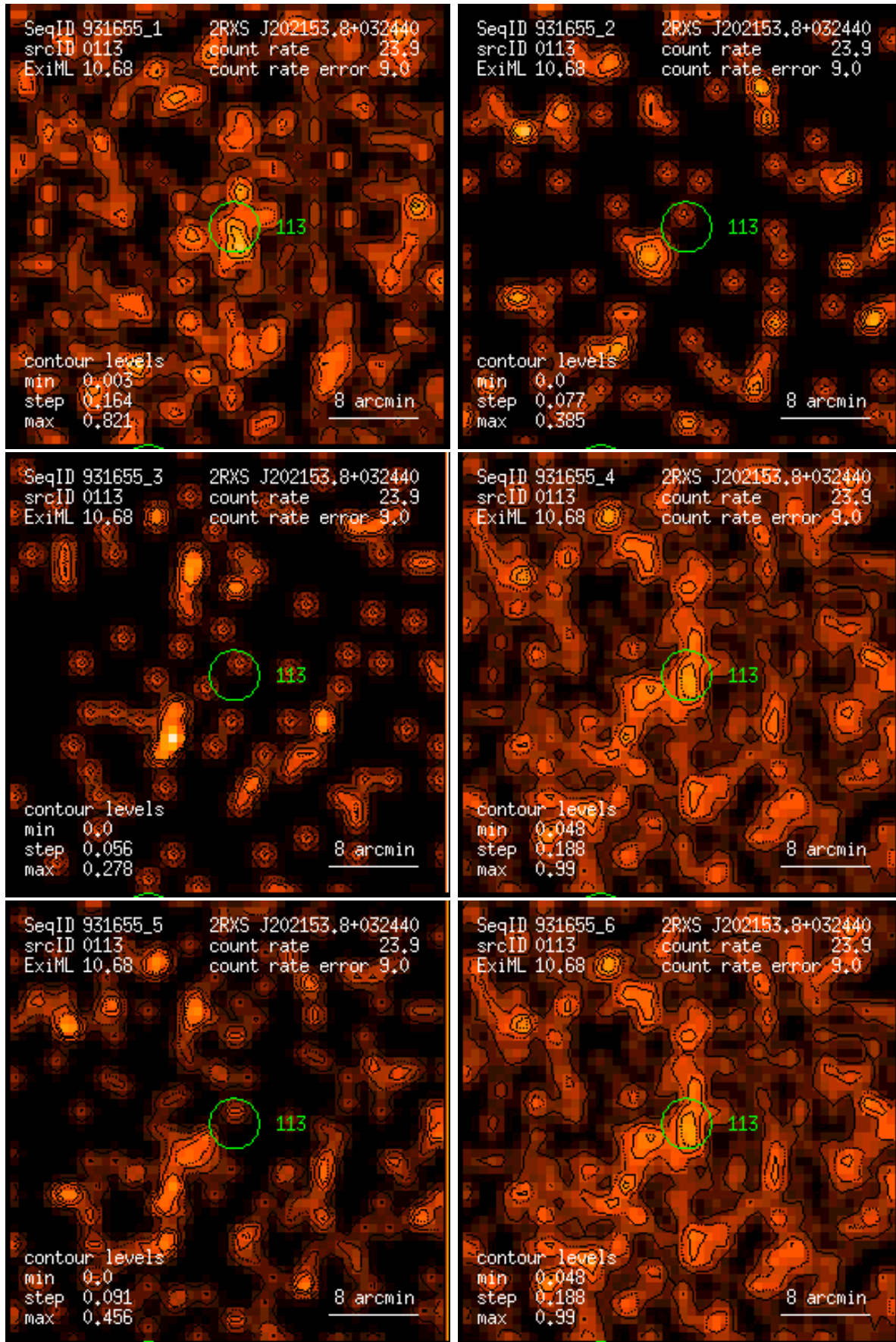
Figure 113: RASS 931655: detection 0113: band rate images, Gaussian filter: (1) PSPC channels 11 – 41, (2) 52 – 90, (3) 91 – 201, (4) 11 – 235, (5) 52 – 201, (6) 11 – 201. Broad band rates in counts/ks. Band rate contour levels in counts/ks/arcmin 2 .
