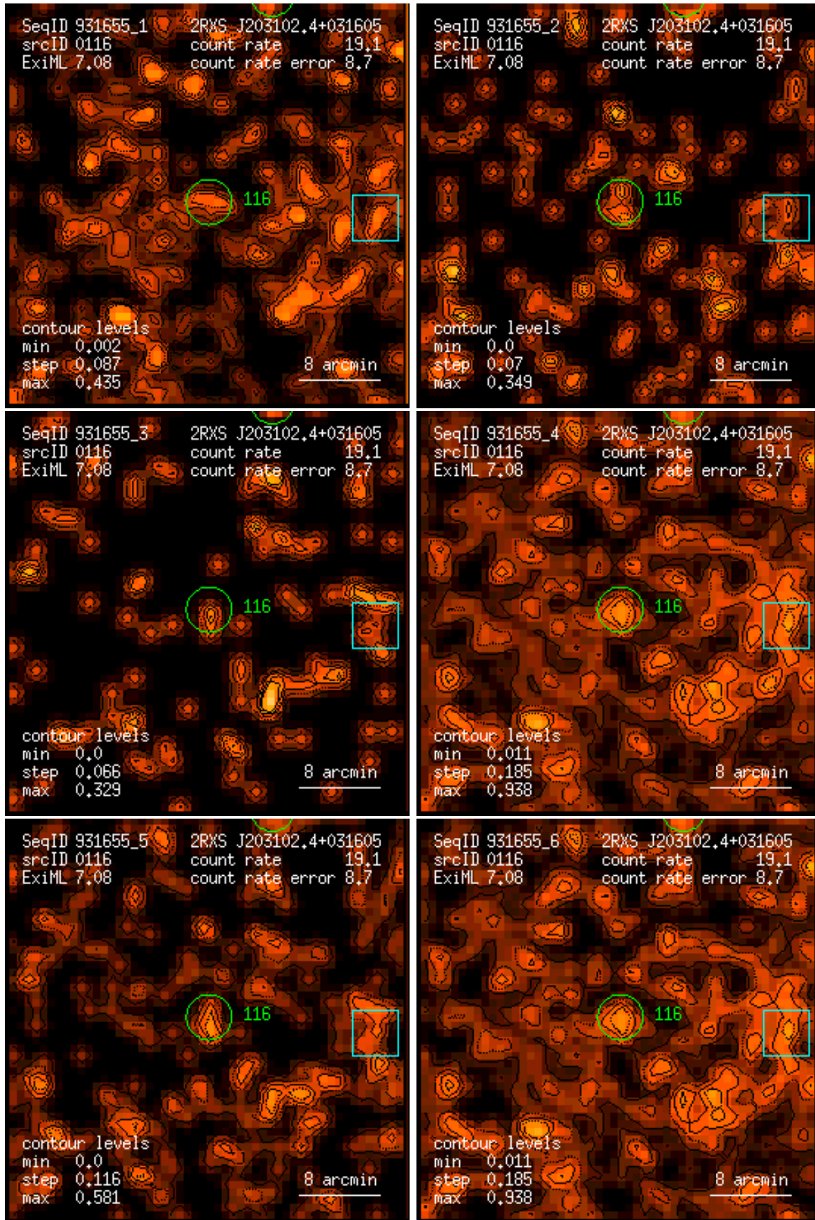
Figure 116: RASS 931655: detection 0116: band rate images, Gaussian filter: (1) PSPC channels 11 – 41, (2) 52 – 90, (3) 91 – 201, (4) 11 – 235, (5) 52 – 201, (6) 11 – 201. Broad band rates in counts/ks. Band rate contour levels in counts/ks/arcmin 2 .
