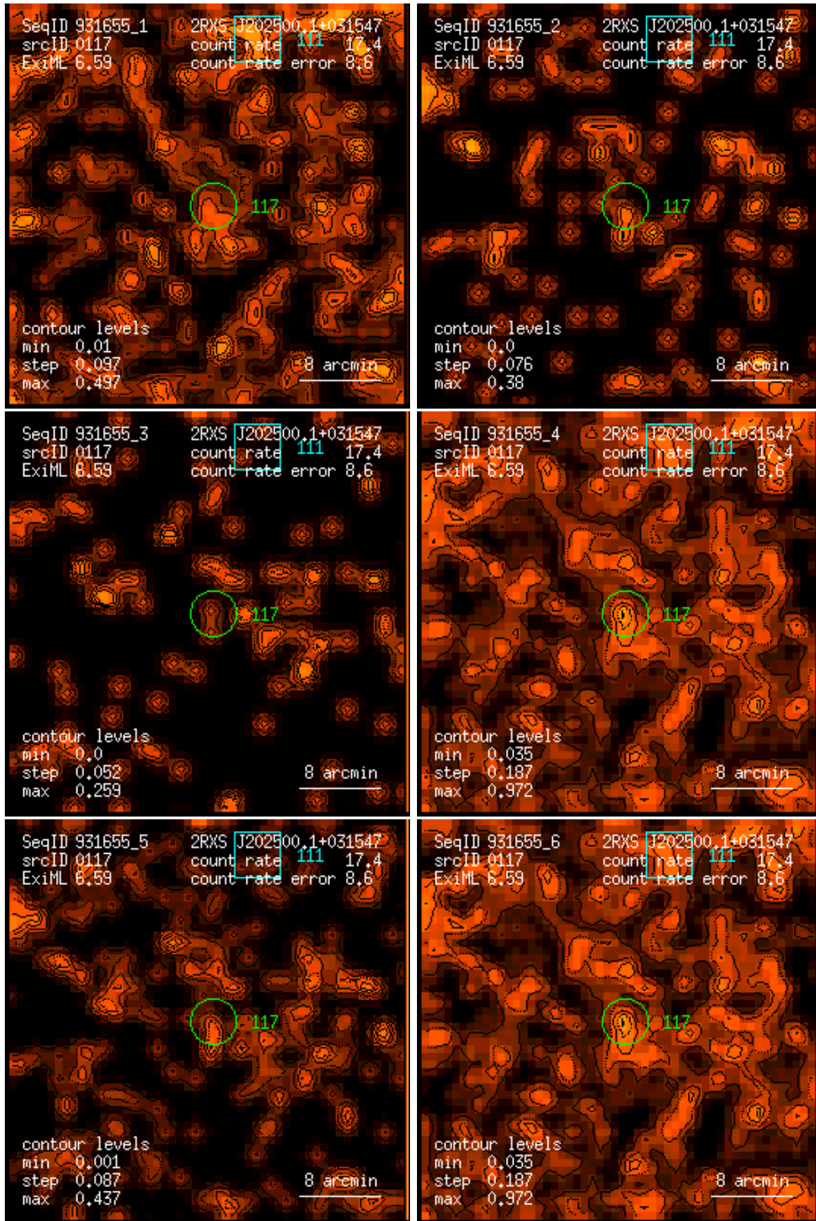
Figure 117: RASS 931655: detection 0117: band rate images, Gaussian filter: (1) PSPC channels 11 – 41, (2) 52 – 90, (3) 91 – 201, (4) 11 – 235, (5) 52 – 201, (6) 11 – 201. Broad band rates in counts/ks. Band rate contour levels in counts/ks/arcmin 2 .
