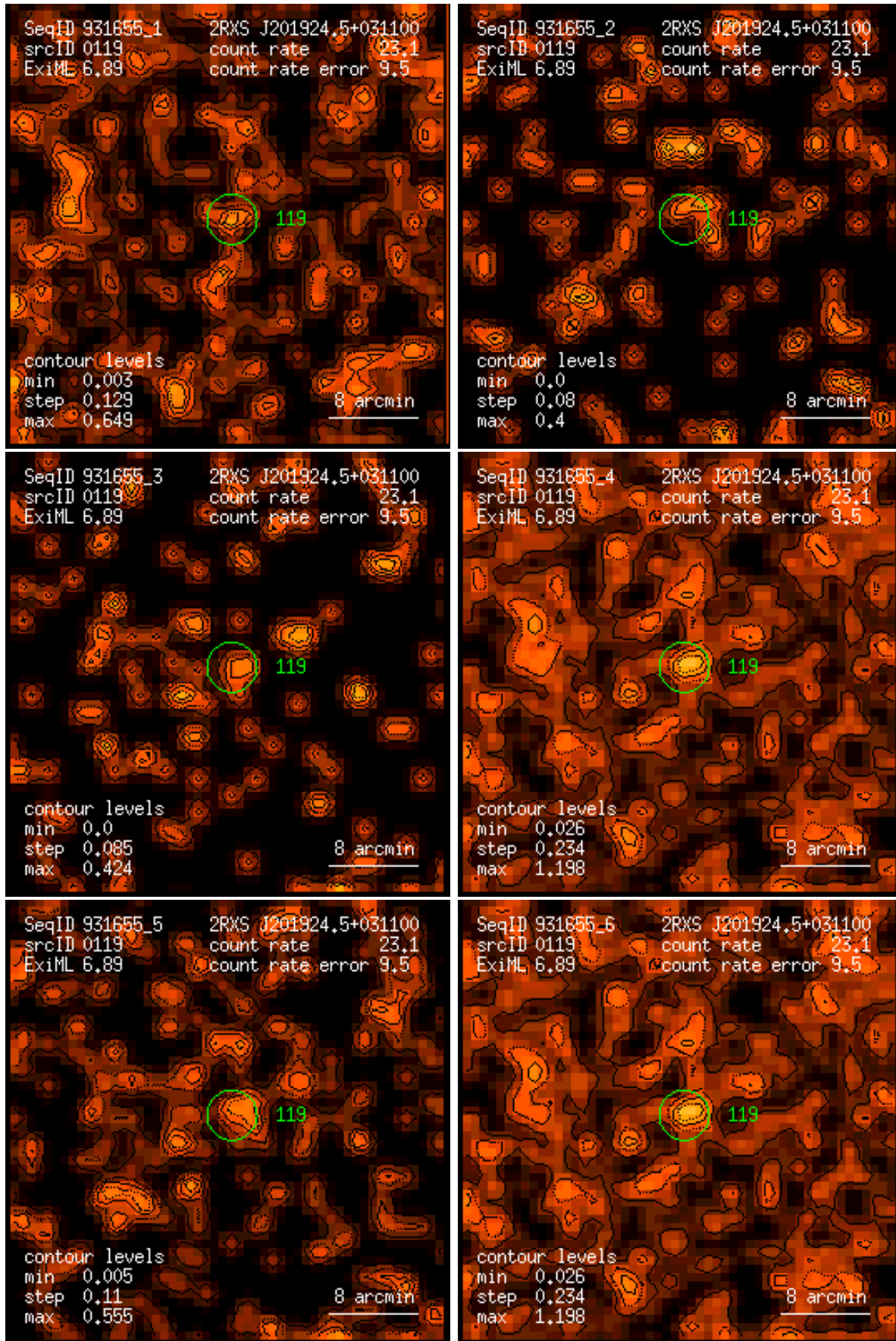
Figure 119: RASS 931655: detection 0119: band rate images, Gaussian filter: (1) PSPC channels 11 – 41, (2) 52 – 90, (3) 91 – 201, (4) 11 – 235, (5) 52 – 201, (6) 11 – 201. Broad band rates in counts/ks. Band rate contour levels in counts/ks/arcmin 2 .
