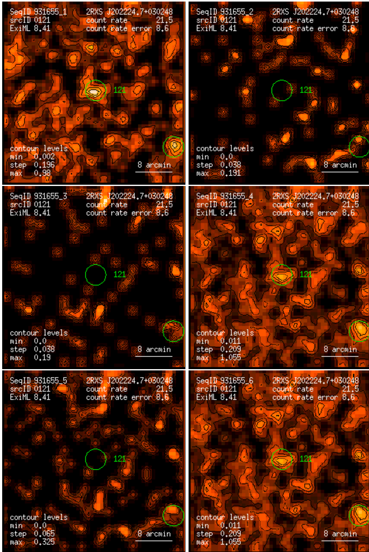
Figure 121: RASS 931655: detection 0121: band rate images, Gaussian filter: (1) PSPC channels 11 – 41, (2) 52 – 90, (3) 91 – 201, (4) 11 – 235, (5) 52 – 201, (6) 11 – 201. Broad band rates in counts/ks. Band rate contour levels in counts/ks/arcmin 2 .
